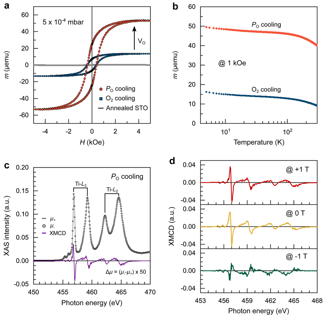
FIG. 5. (a) Comparison of the 5 K magnetic hysteresis loops of the B-site cation deficient STO films, grown at P_O = 5 \times 10^{-4} mbar, with different cooling processes, i.e., after film growth, the two samples were cooled in a high O_2 atmosphere (blue circle, O_2 cooling) and in the same growth pressure (red circle, P_O cooling) separately. The hysteretic magnetic responses of the two STO/STO samples are compared with a non-magnetic annealed TiO_2 -STO(001) substrate. (b) Variable temperature magnetic moments of the samples, prepared by different cooling processes. A constant magnetic field of 1 kOe was applied to the samples during the temperature measurements. (c) XAS and XMCD across the Ti L_{2,3} -edges of the B-site cation deficient STO film sample with P_O cooling as measured at 4 K. (d) Ti L_{2,3} XMCD of the same STO thin film as measured by sweeping the applied magnetic fields (+1 T \rightarrow 0 T \rightarrow -1 T).
