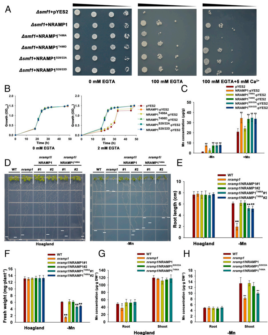
Fig. 4. Functional analysis of NRAMP1 phosphorylated by CPK21/23. (A) Empty vector ( \Delta smf1 +pYES2), NRAMP1 ( \Delta smf1 +NRAMP1), and NRAMP1 variants ( \Delta smf1 +NRAMP1 variants) were transferred into the yeast mutant strain \Delta smf1 . Yeast cells were grown on medium SD-U (without uracil), SD-U added 100 mM EGTA (Mn 2+ chelator), and SD-U added 100 mM EGTA and 5 mM CaCl 2 . (B) Growth curves of yeast cells expressing pYES2, NRAMP1, and NRAMP1 variants were plotted from OD 600 values. Growth of yeast cells in liquid cultures containing 0 or 2 mM EGTA was monitored every 3 h from 18 to 51 h (data are means \pm SD n = 3 biological replicates). (C) ICP-MS analysis of Mn concentration in yeast cells carrying empty vector, NRAMP1, and NRAMP1 variants. The yeast cells grown on liquid medium SD-U and SD-U added 2 mM EGTA for 24 h. Data are means \pm SD n = 6; * P < 0.05, ** P < 0.01; Student's t test). (D) Mn-deficiency phenotypes of ProNRAMP1:NRAMP1 and ProNRAMP1:NRAMP1 T498A transgenic plants. These plants were grown on Mn-replete conditions and Mn-free conditions. (E) Statistical analysis of root lengths of plants shown in D ( n = 16 seedlings; ** P < 0.01; Student's t test). (F) Statistical analysis of fresh weight of plants shown in D ( n = 16 seedlings; ** P < 0.01; Student's t test). (G) Statistical analysis of Mn concentrations of plants under Hoagland medium shown in D ( n = 3 biological replicates; * P < 0.05; Student's t test). (H) Statistical analysis of Mn concentrations of plants under Mn deficiency shown in D ( n = 3 biological replicates; ** P < 0.01; Student's t test).
