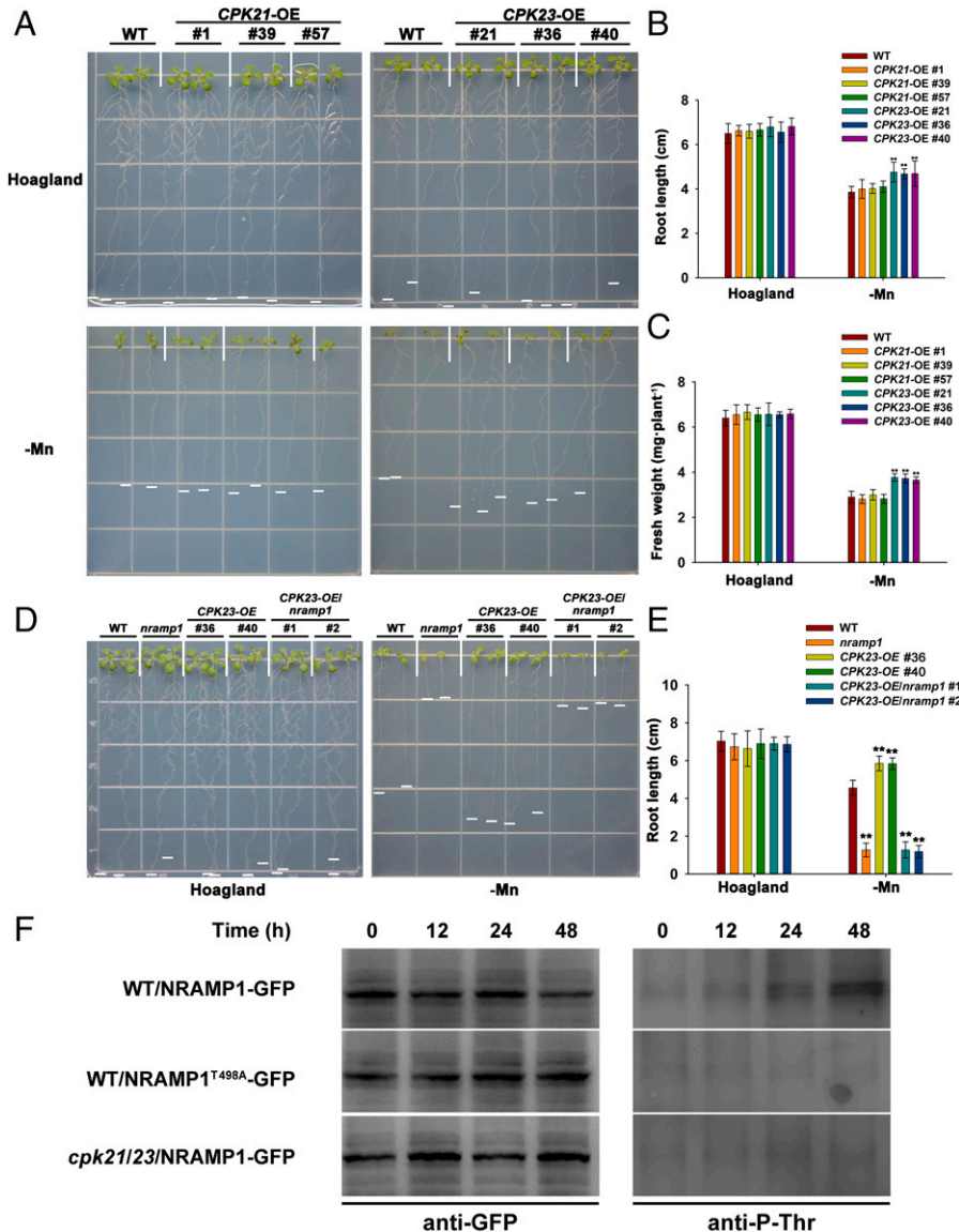
Fig. 5. Genetic interaction of CPK21/23 with NRAMP1. (A) Mn-deficiency phenotypes of CPK21 -OE plants. The plants were grown on Mn-replete conditions and Mn-free conditions. (B) Statistical analysis of root lengths of plants shown in A ( n = 16 seedlings; **P < 0.01 ; Student's t test). (C) Statistical analysis of fresh weight of plants shown in A ( n = 16 seedlings; **P < 0.01 ; Student's t test). (D) Mn-deficiency phenotype of CPK23 -OE/ nramp1 . (E) Statistical analysis of primary root lengths of plants shown in D ( n = 16 seedlings; **P < 0.01 ; Student's t test). (F) The seedlings were treated with Mn-deficient conditions for 0, 12, 24, and 48 h, respectively. The signal of NRAMP1 and GFP were detected by P-Thr antibody and GFP antibody, respectively.
