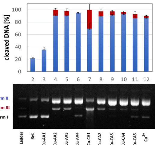
Fig. 8 DNA cleavage activity of complexes Cu-AA1–CuAA4, Cu-CA1–Cu-CA5 and CuCl 2 at 35 μM (agarose gel). Incubation was done using 0.025 μg μL –1 plasmid DNA pBR322, 50 mM MOPS buffer (pH 7.4) and 1 mM ascorbate for 1 h at 37 °C and 500 rpm (same conditions for the reference without addition of a complex). Error bars for the standard deviation were obtained with at least three experiments. Blue bars indicate percentage of form II, red bars percentage of form III. The ladder contains plasmid DNA form I, II and III enzymatically prepared for band referencing.
