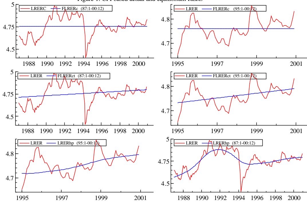
Figure 1: CPI based actual and equilibrium RERs
