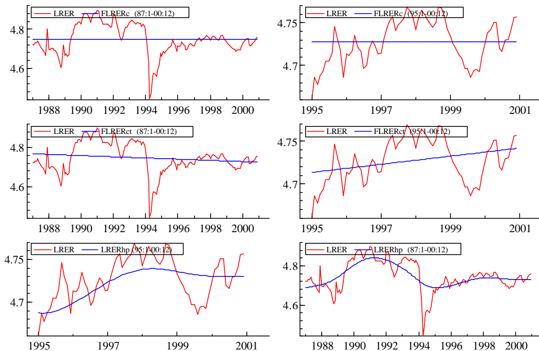
Figure 3: WPI based actual and equilibrium TWREr
