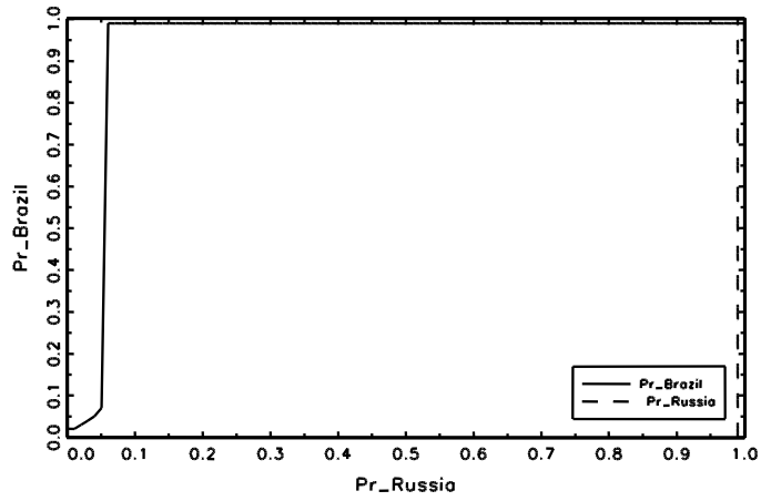
Figure 10: Brazil - Russia 1999
