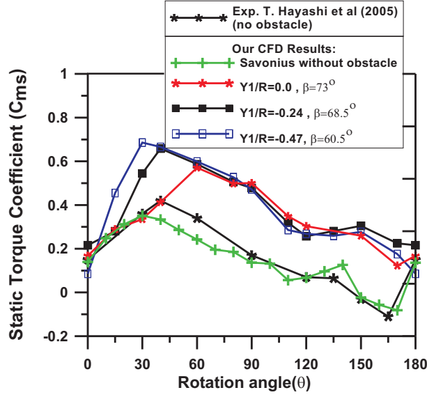
Figure 6.29: Static torque coefficient as a function of the rotor angle \theta for three different values of Y_1 choosing X_1/R = -1.4 and X_2/R = -1.76 .
