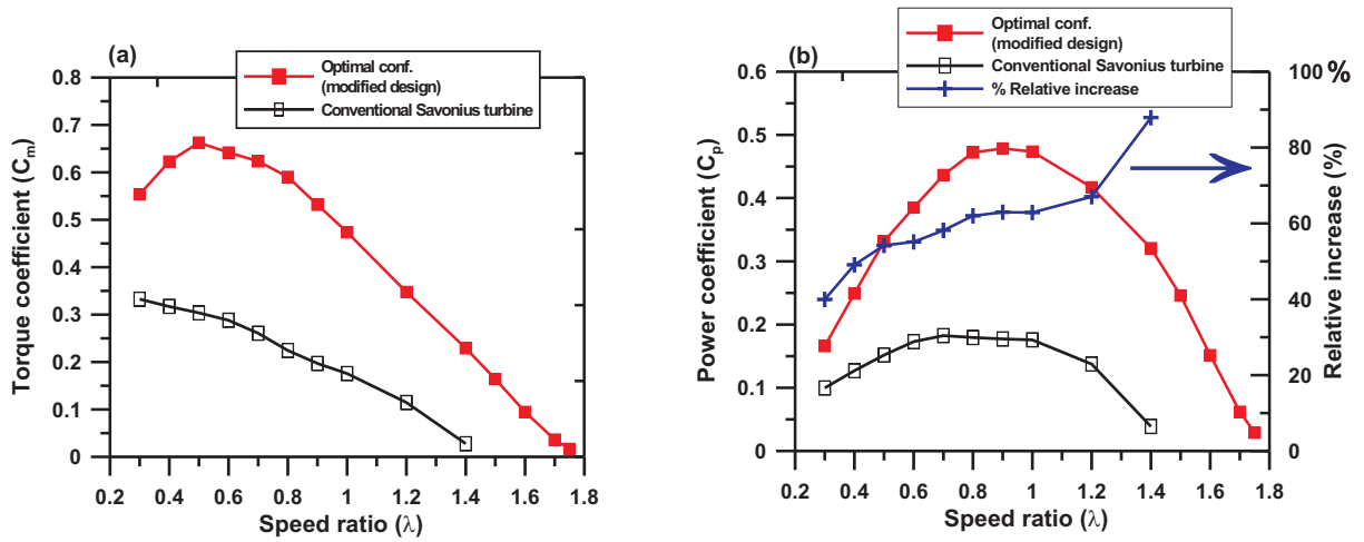
Figure 6.49: Performance of the optimized configuration (red line) compared to the conventional Savonius turbine (black line): a: torque coefficient; b: power coefficient. The corresponding relative increase compared to the classical configuration is shown with blue line.
