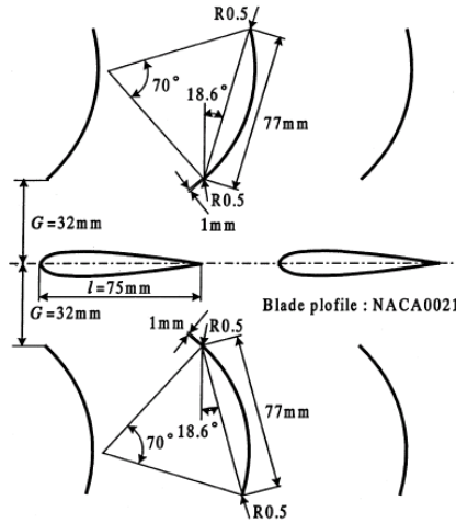
Figure 3.19: Installation of guide vanes [106].
