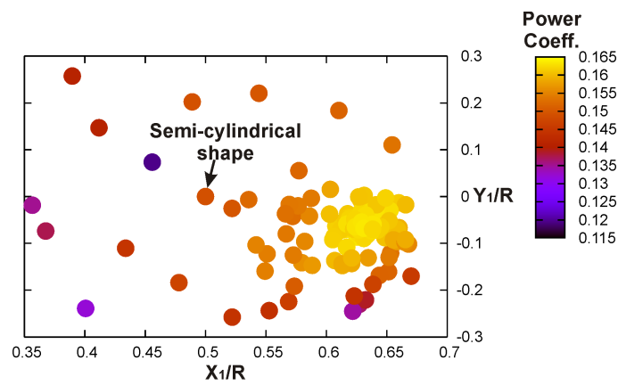
Figure 6.10: The two input parameters of the optimization and the power coefficient.
