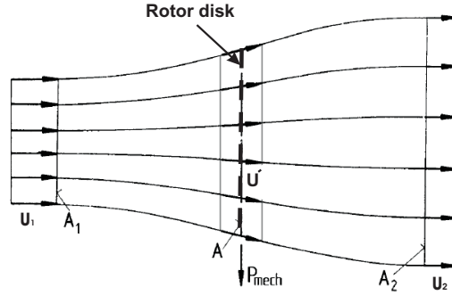
Figure 2.5: Flow conditions due to the extraction of mechanical energy from a free-stream air flow, according to the elementary momentum theory.
