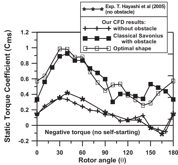
Figure 6.37: Static torque coefficient C_{ms} as a function of the fixed rotor angle \theta for the optimal configuration compared to the standard Savonius turbine with and without obstacle plate. For this last case, the experimental results of [38] are also shown for comparison.
