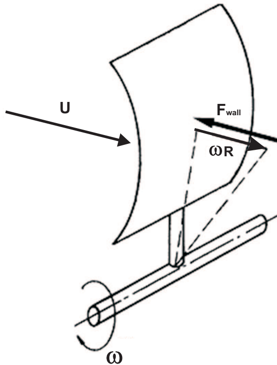
Figure 2.4: Flow conditions and drag force for vertical axis turbines [53].
