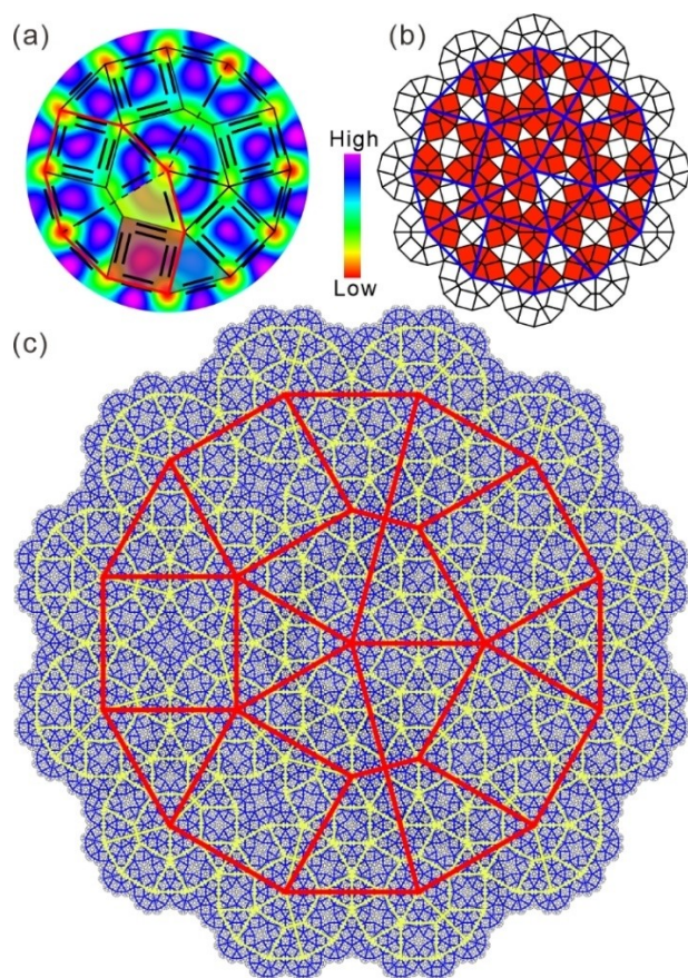
Figure 4. a) Reconstructed ED map of a patch of a hypothetical approximatant of the CLQC phase with an extra-large p4gm^L lattice ( p4gm^{xl} with a_{squ} = 32.53 nm). High ED is shown in purple and low ED is in red. The black thick lines represent the aromatic cores while the red line indicates an octagonal motif; b) CLQC tiling inflated once according to the inflation rule; [10] the octagonal motifs are highlighted by red color; c) 3rd generation of inflation, see Section S4.2 for details.
