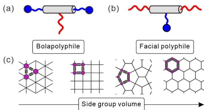
Scheme 1. (a, b) Schematic representations of the basic structures of the T-shaped polyphiles and (c) examples of polyagonal honeycombs (cuts perpendicular to the prismatic cell long axis), representing tilings with congruent tiles; [7a] side-by-side pairs of the rod-like units (black thick lines) form the walls of the polyagonal cells, while the end groups form the nodes (purple circles) and the side groups fill the interior.
