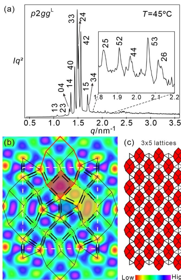
Figure 7. a) SAXS diffractogram of the p2gg^L phase of compound 12/5 at 45 °C upon second heating; b) the reconstructed ED map (see also Figure S15b), molecular packing and tiling of the p2gg^L phase. The tiling is composed of non-regular trapezoids, squares, triangles, and pentagons; c) a collection of 15 lattices. The highlighted octagonal motifs are parallel with each other and separated by deformed trapezoids and triangular tiles. For more details, see Table S5.
