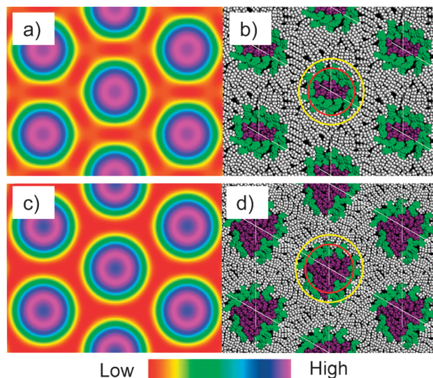
Fig. 6 Electron density maps of the \text{Col}_{\text{hex}} phases of (a) compound 3^{12}(\text{OH})_2 and (c) compound 3^{12}\text{EO}^3(\text{OH})_2 as reconstructed from the synchrotron powder diffraction patterns (color code: purple/blue = high, green/yellow = medium and red = low electron density; for details of the reconstruction, see the ESI†); (b) snapshot of the structure of the \text{Col}_{\text{hex}} phase of 3^{12}(\text{OH})_2 and (d) of 3^{12}\text{EO}^3(\text{OH})_2 after MD annealing (polar groups are colored purple and the aromatic cores green, alkyl chains gray); red and yellow circles represent the boundaries between high and medium and medium and low electron density regions in the electron density maps, respectively.
