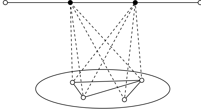
FIGURE 5.2. Appending a threshold graph to a split graph
