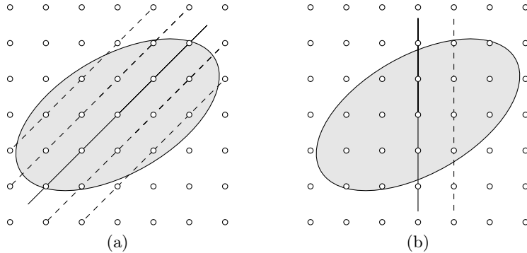
FIGURE 3.6. A lattice line through the origin that (a) has the property of Lemma 3.28 and (b) one that does not.
