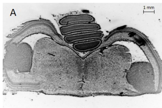
Fig. 6 [ ^{68}\text{Ga} ]FAPI-46 of a chick embryo on EDD 19. (A) 4',6-diamidino-2-phenylindole (DAPI) image of U87 IDH1 R132H intracerebral tumour showing densely packed solid tumour cells in the ventricles
