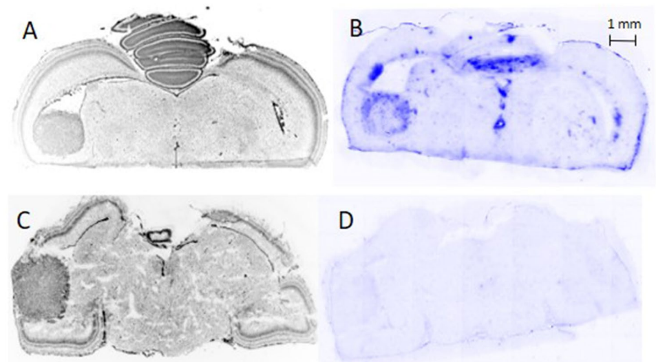
Fig. 3 Two representative EDD 19 chick embryo brains with U87-MG tumours showing a disrupted (A,B) and an intact (C,D) blood-tumour-barrier. A,C: 4',6-diamidino-2-phenylindole (DAPI) staining shows densely packed tumour cells in the tectum opticum. B,D: Consecutive slices of A and C, respectively, with (B) and without (D) Evans blue dye extravasation in the tumour region, thus indicating a disrupted (B) and an intact (D) blood-tumour-barrier.
