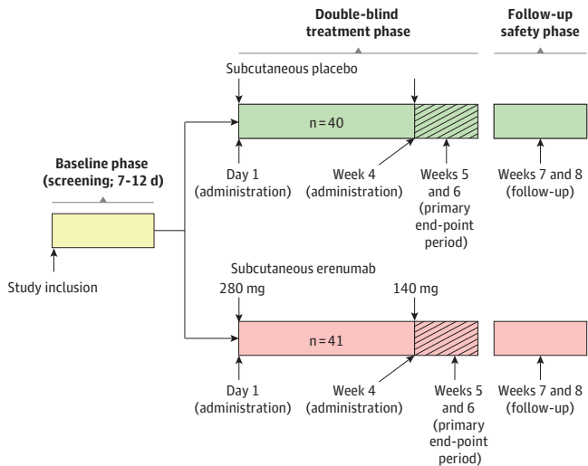
Figure 2. Study Design
