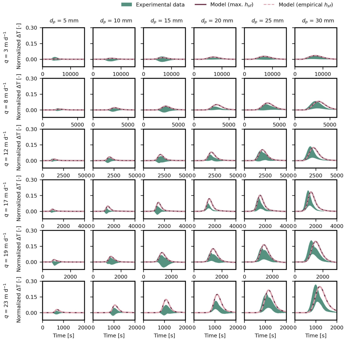
Figure 4. Summary of experimental data and model results with estimated heat transfer coefficient, empirical h_{sf} , and the possible maximum heat transfer coefficient, \max. h_{sf} , for six different grain sizes and six different flow velocities. The green shaded area demonstrates the range between minimal and maximal \Delta T(t) measured for a specific grain size and a specific flow velocity from the laboratory experiments by Lee et al. (2025). The pink dashed line indicates the \Delta T(t) range from the model results with the estimated empirical h_{sf} by the correlation of Gossler et al. (2020). The dark red solid line presents the modeled \Delta T(t) with \max. h_{sf} .
