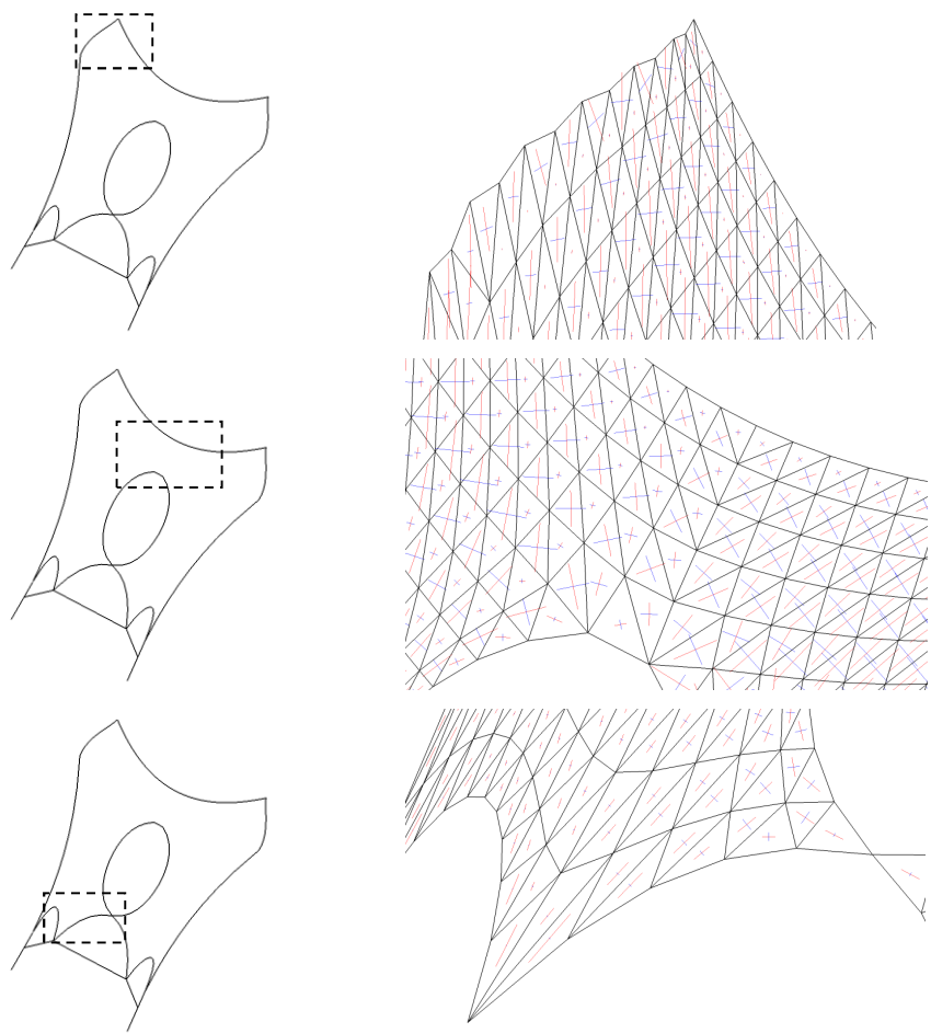
ULS stresses: SI and SII directions, P+DL+S configuration
