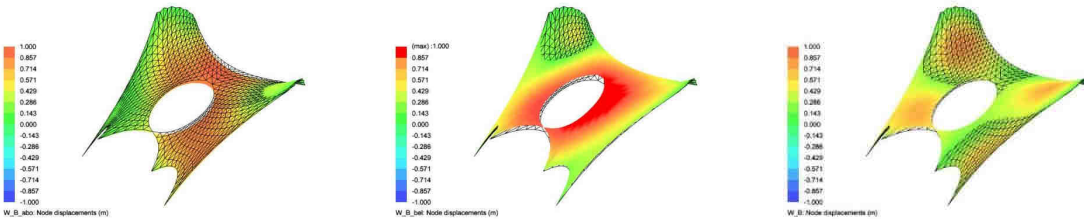
W_B deflections: above, below then cumulated
