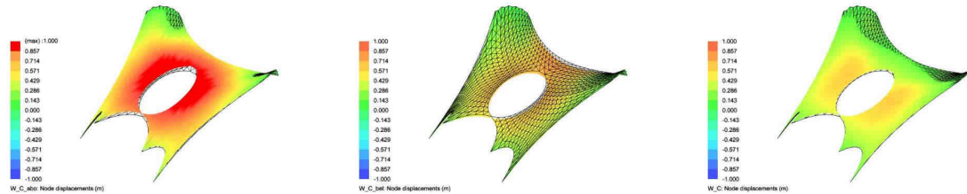
W_C deflections: above, below then cumulated
