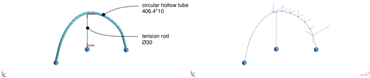
Structure and loads transferred in steel software
