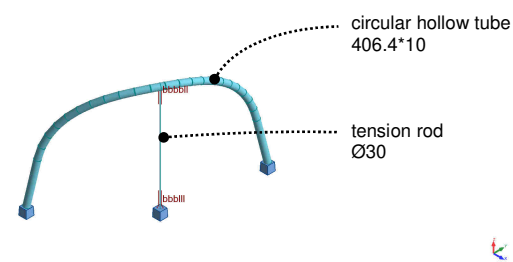
Structure and loads transferred in steel software
