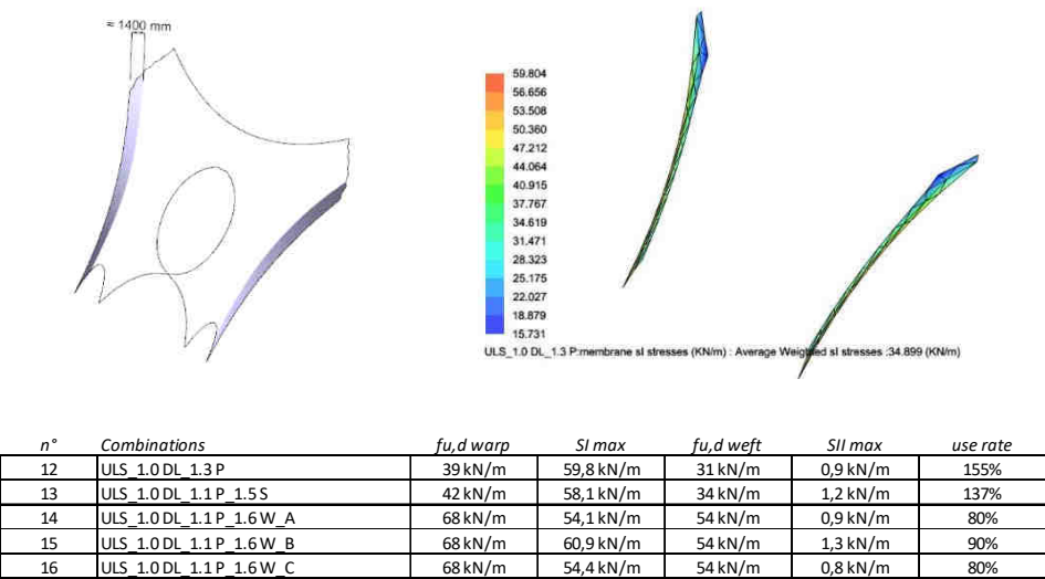
ULS stresses: reinforcements areas
