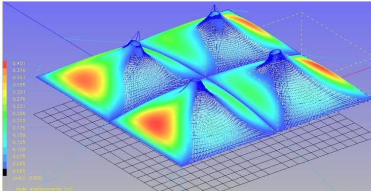
Image 80 : Membrane Deformation
