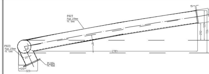
Pipe connection
