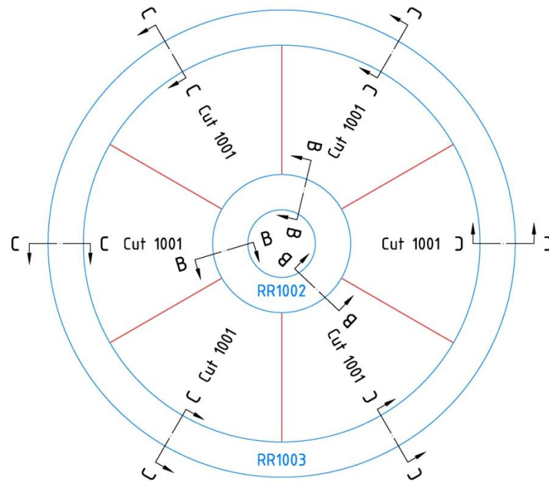
Image 108 : Plan View
