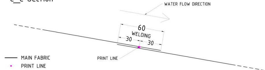
C_C Section
