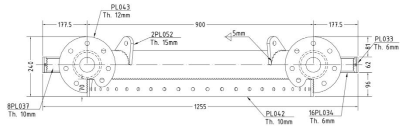
Left View
