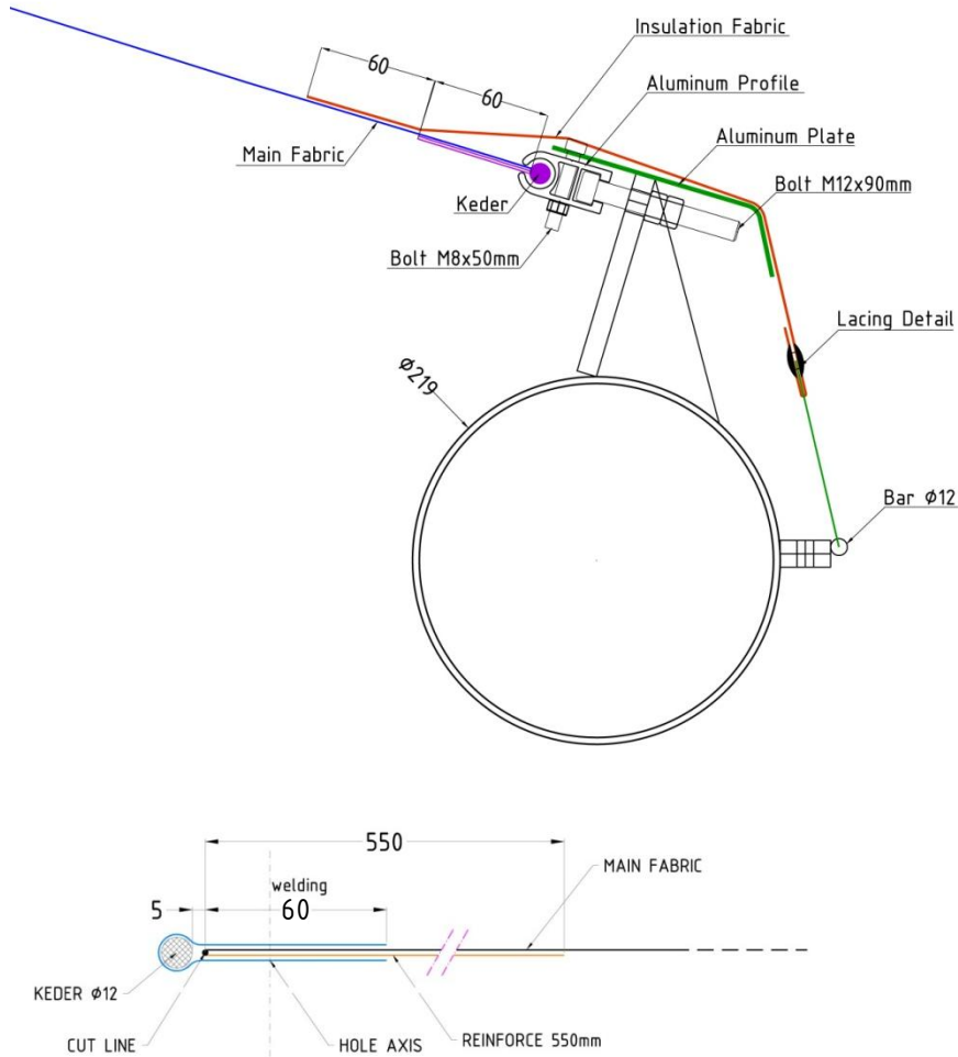
B_B Section
