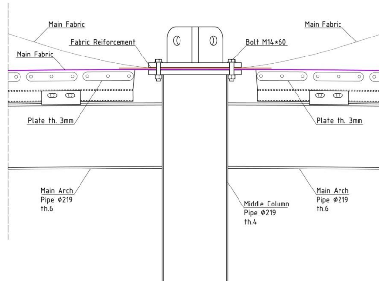
D_D Section
