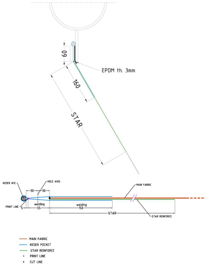
E_E Section
