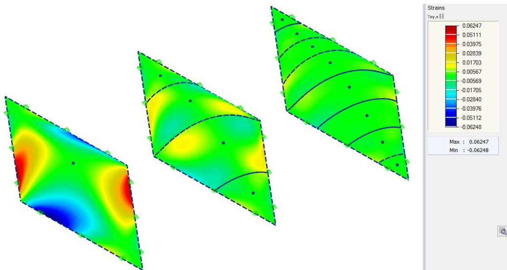
Fig. 147 – Strains \varepsilon_{xy} in 2D patterns caused by flattening
