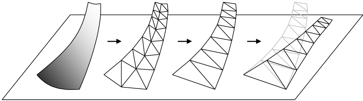
Fig. 134 – The basis of the simple triangulation method (from the left: the spatial shape, the FE mesh of the spatial model used for form-finding and structural analysis purposes, the modified mesh for flattening purposes, the flattened pattern) [19]
