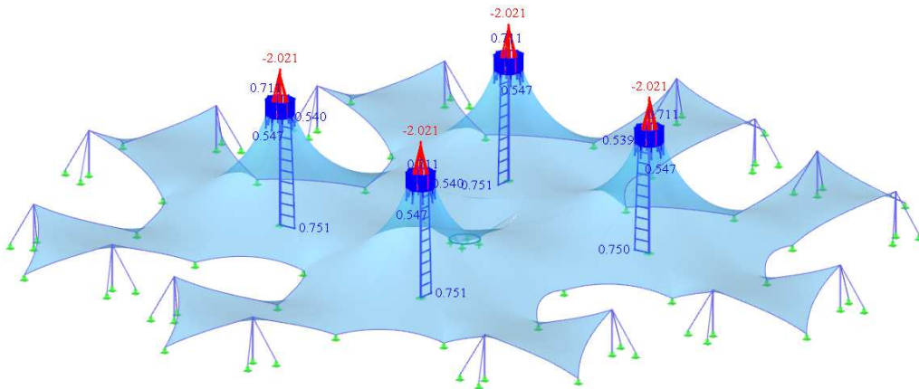
Fig. 50 – Bending moments M_y
