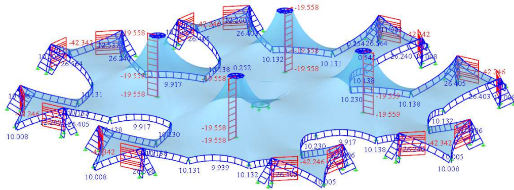
Fig. 49 – Normal forces N
