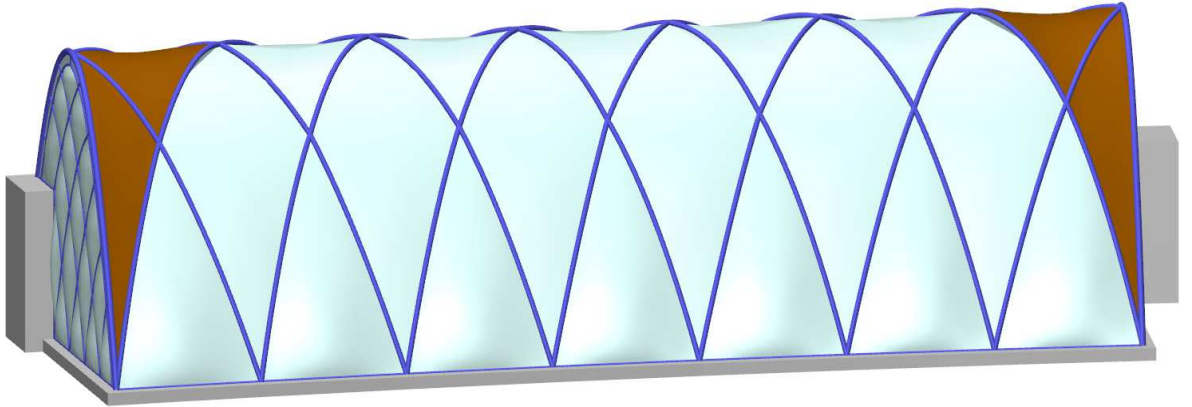
Fig. 117 – Geometry of the greenhouse structure
