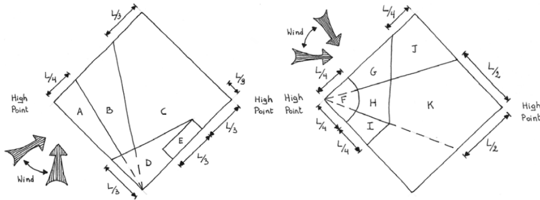
Fig. 86 – C_p zones definition on the hyper structure [35]
