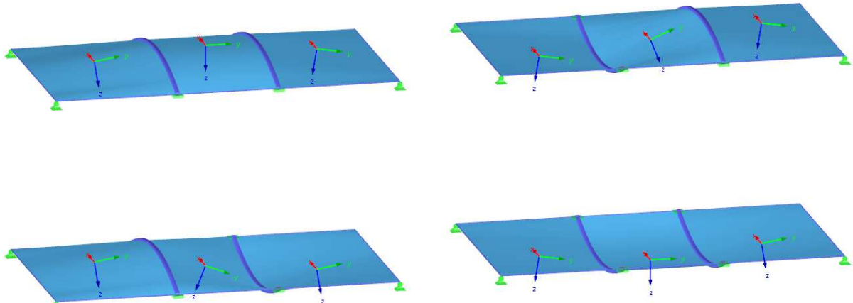
Fig. 75 – Different initial shapes of the membrane structures with the warp/weft orientation displayed
