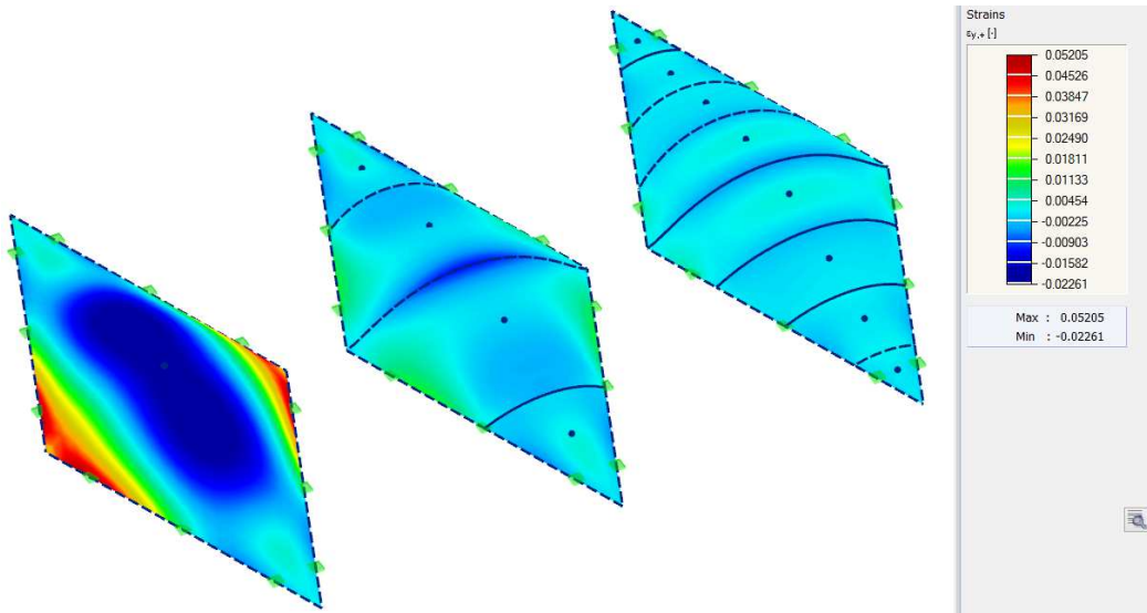
Fig. 146 – Strains \varepsilon_y in 2D patterns caused by flattening
