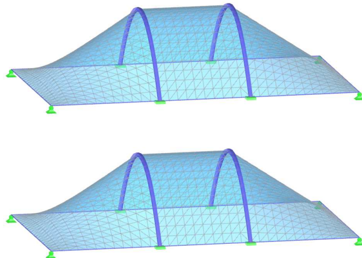
Fig. 69 – FE mesh of the membrane structures in the initial position, the structure with (above) and without (bellow) the analysis of the shape of steel arches
