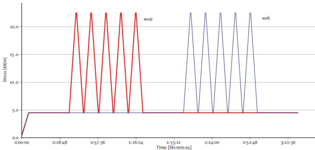
Fig. 137 – Biaxial test: load history [35]
