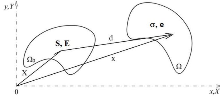
Fig. 78 – Reference (X, \Omega_0) and the current (x, \Omega) configuration of the body
