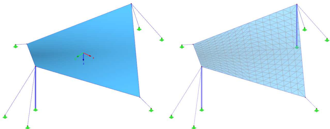
Fig. 5 – Initial shape of a hypar membrane structure with the x/y (warp/weft) orientation displaying (left), FE mesh (right)
