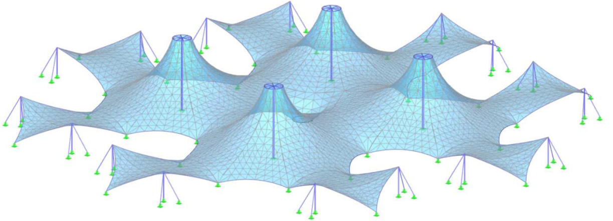
Fig. 154 – FE mesh of the membrane structure
