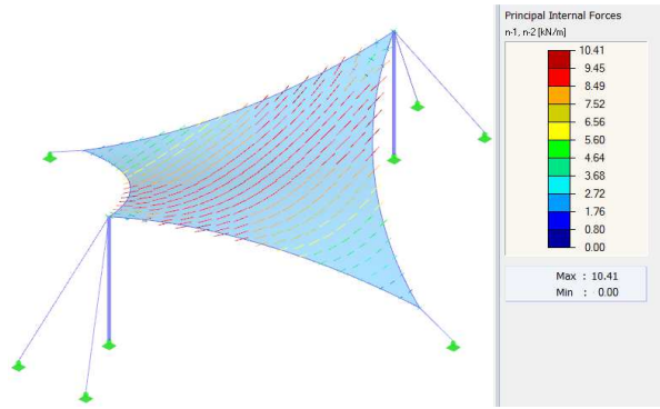
Fig. 99 – Vectors of main internal forces n_1, n_2 (CO18)
