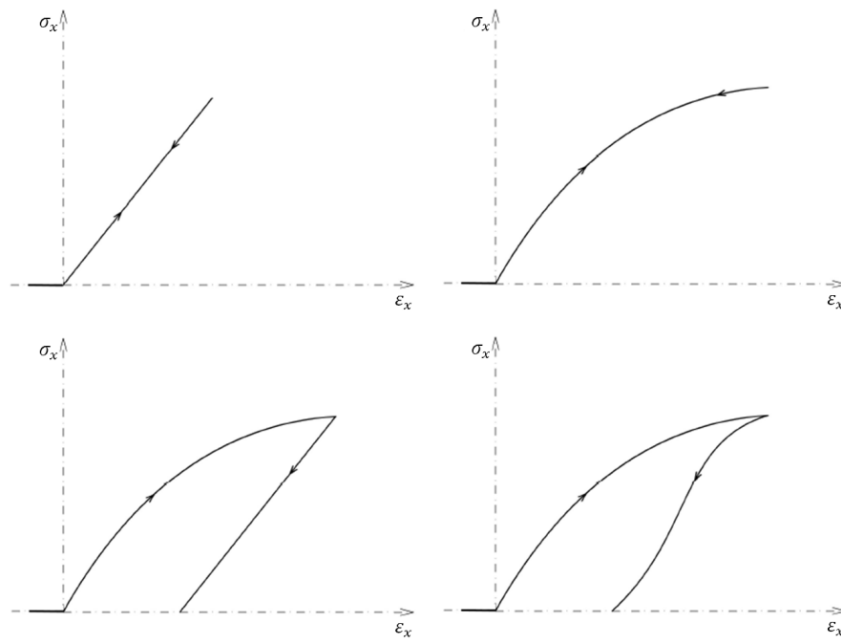
Fig. 80 – Elastic, non-linear elastic, elastic-plastic and general material models
