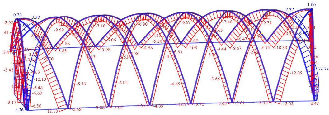
Fig. 38 – Normal forces N
