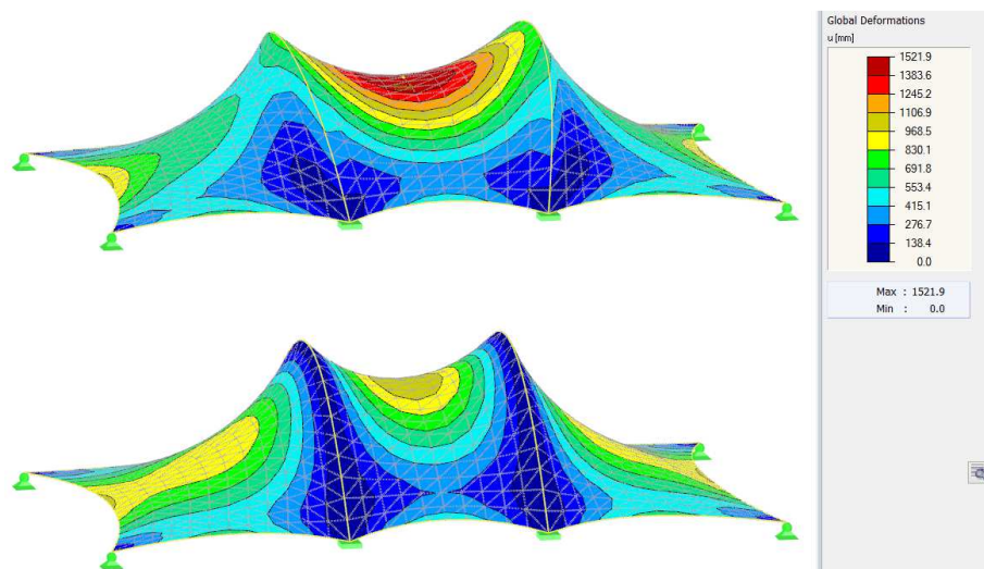
Fig. 70 – Global deformations u during the form-finding, the structure with (above) and without (bellow) the analysis of the shape of steel arches
