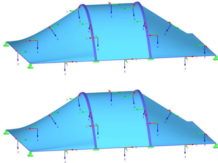
Fig. 68 – Initial shape of the membrane structures displayed with the x/y (warp/weft) orientation and beam axes, the structure with (above) and without (bellow) the analysis of the shape of steel arches
