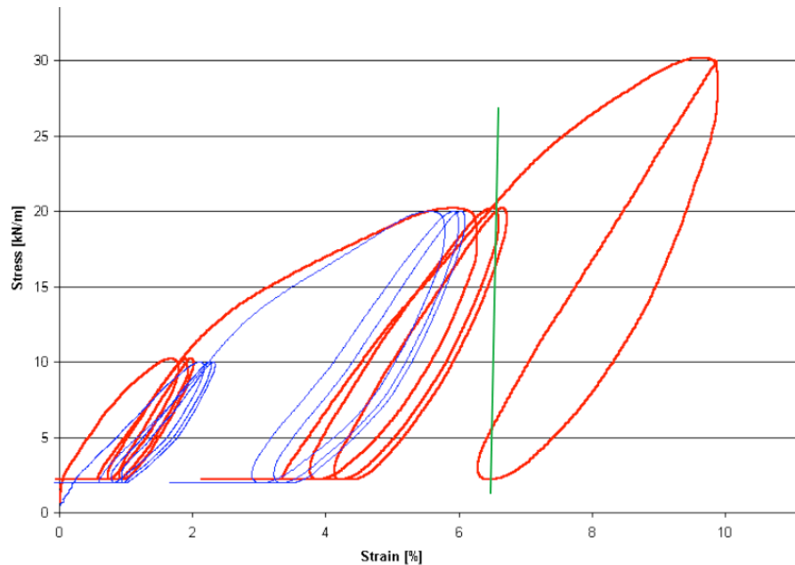
Fig. 139 – Biaxial test: stress-strains diagram [36]
