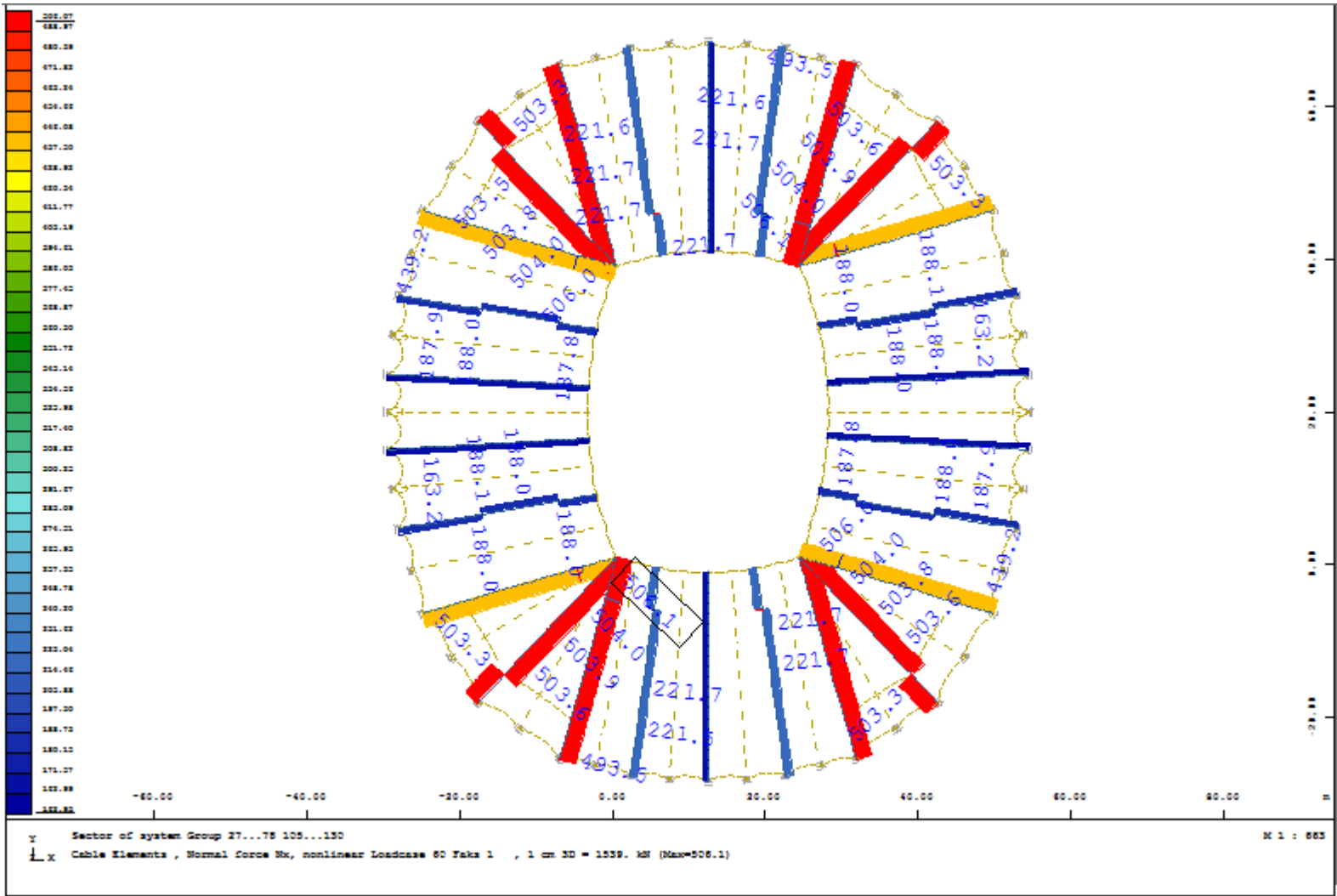
Lower Radial Cables - Prestress
