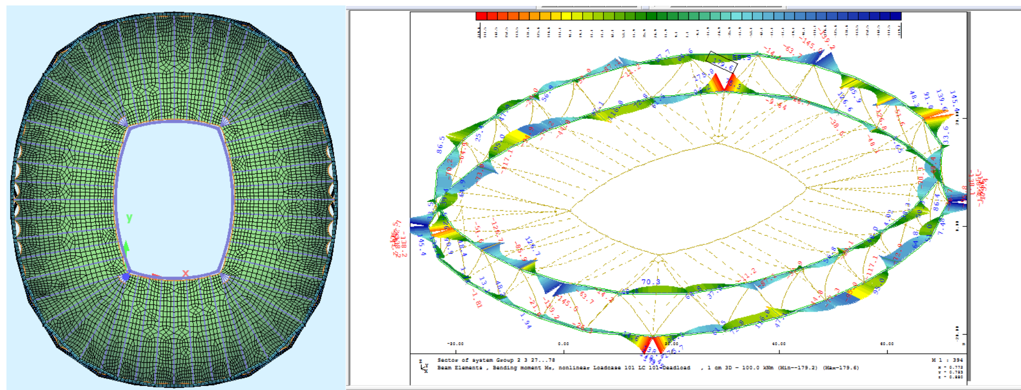
Figure 14 – Corrected Geometry, after Formfinding M_{z,max} = 179 kNm
