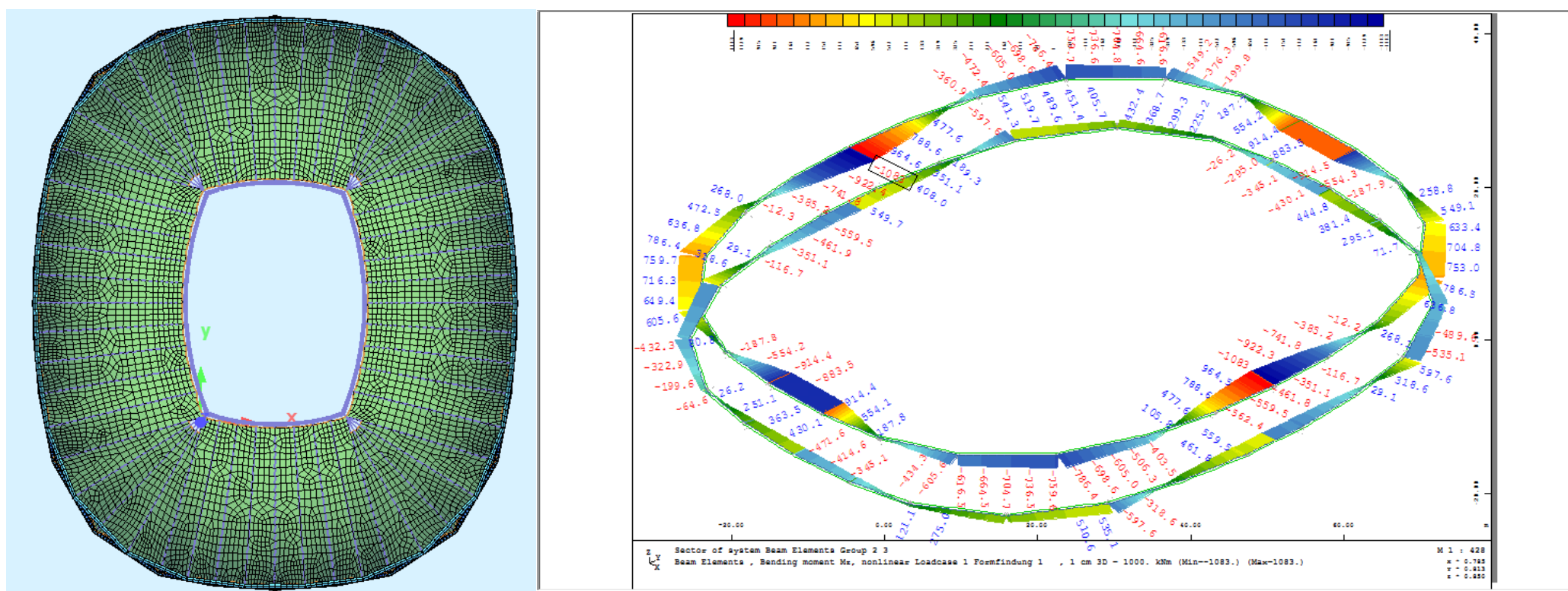
Figure 13 – Initial Geometry, before Formfinding M_{z,max} = 1083 kNm
