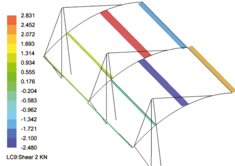
LC9 - Connection beam shear 2 reactions
