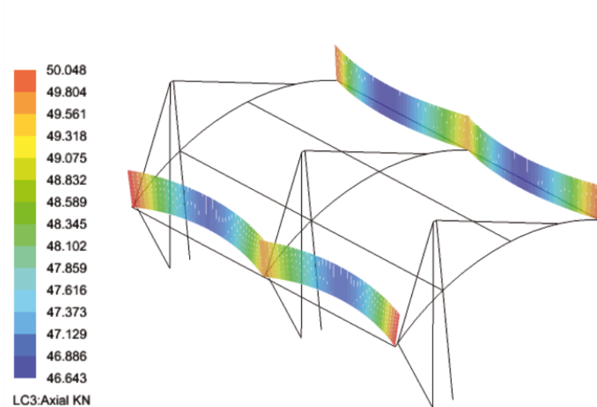
LC3 - Border cable axial reaction
