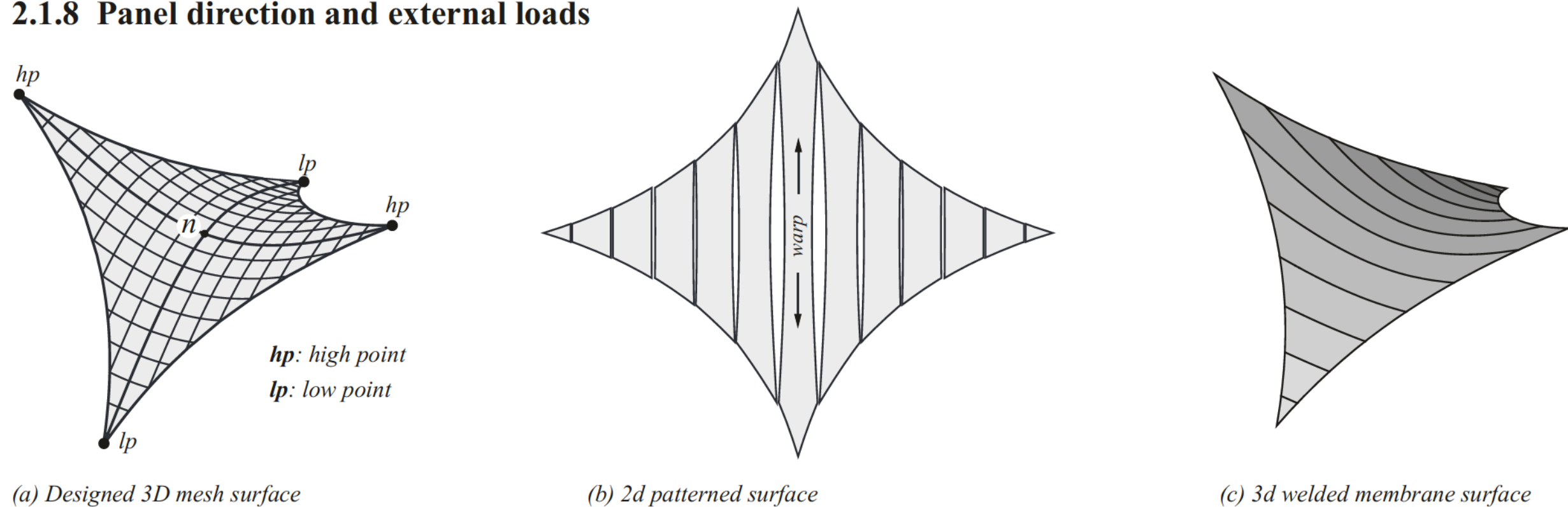
Figure 1.14 Evolution of membrane surface
