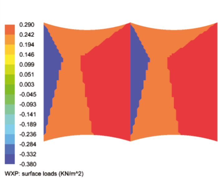
Wind flow from x direction (X+)
