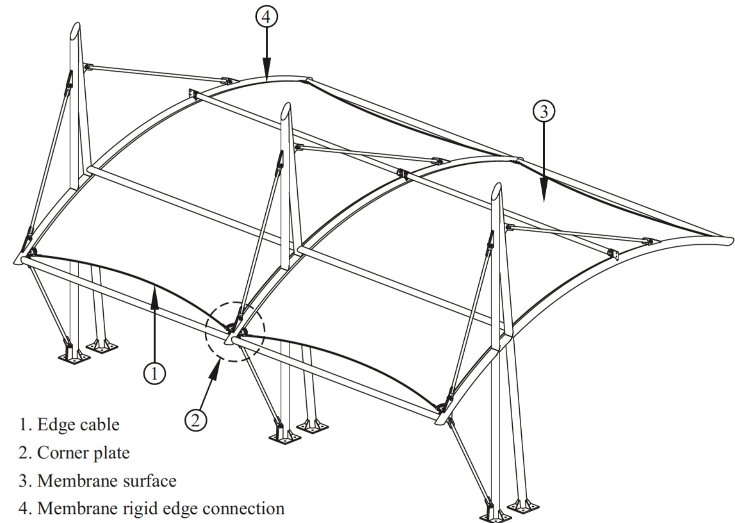
Figure 3.5 3D view of two modules.
