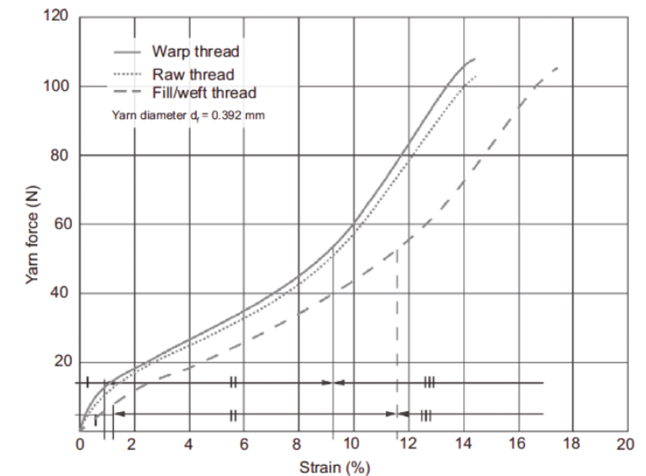
Figure 2.7 Force-strain path of a polyester yarns
