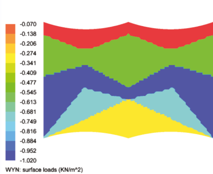
Wind flow from negative y direction (Y-)
