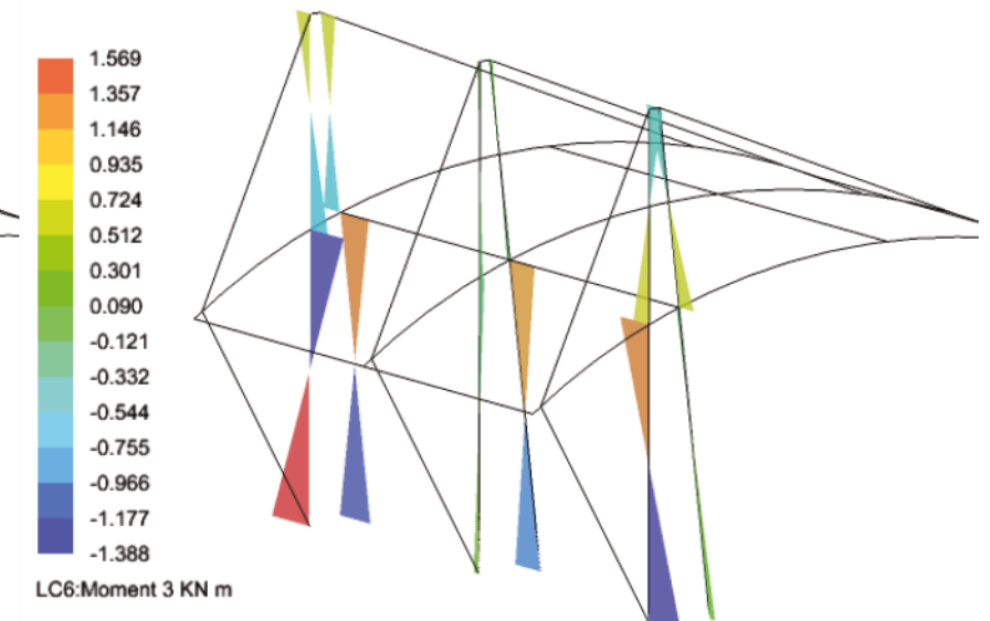
LC6 - Mast M3 reactions
