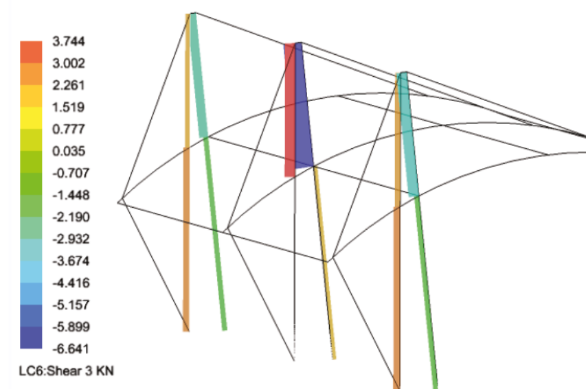
LC6 - Mast shear 3 reactions
