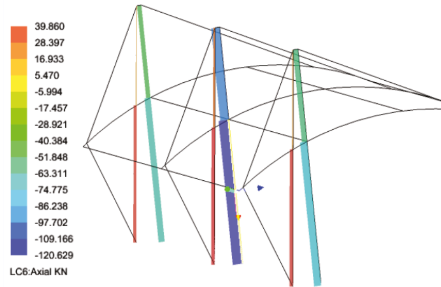
LC6 - Mast axial reactions
