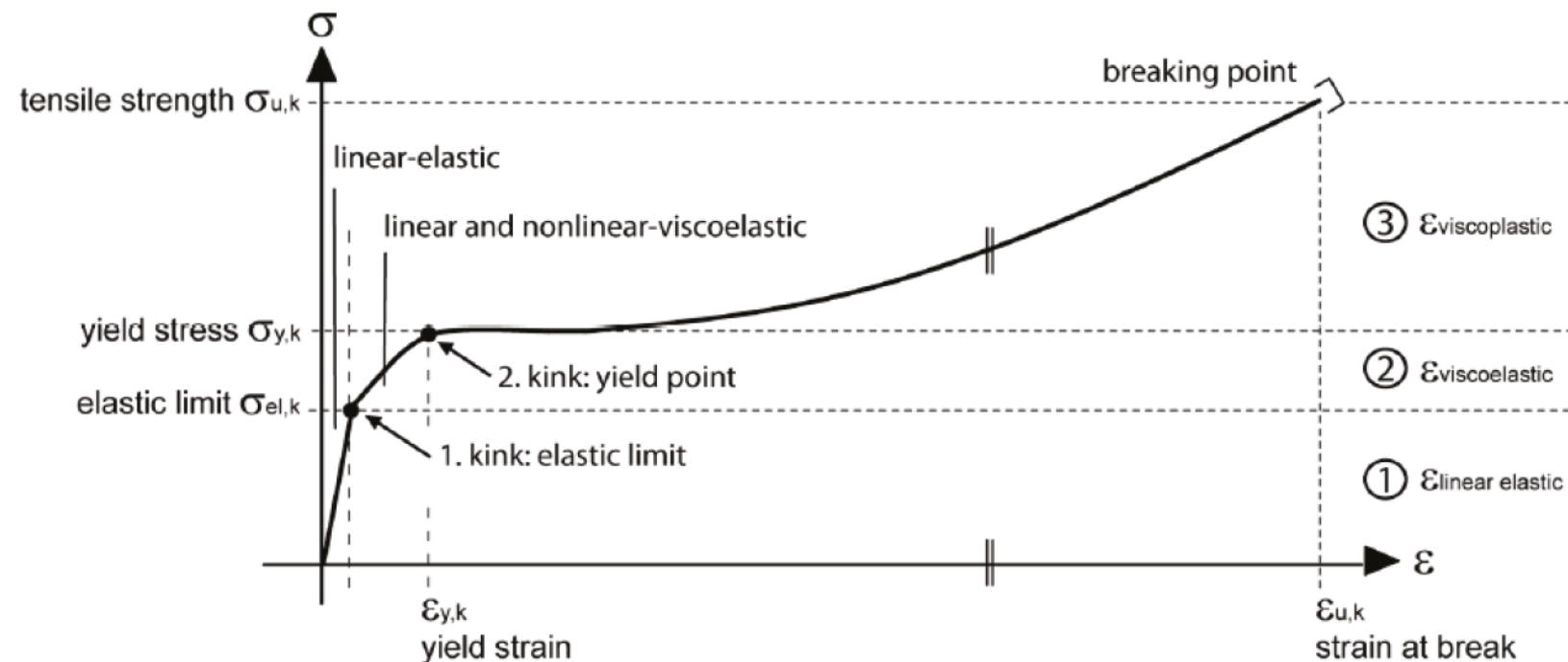
Figure 2.10 Mechanical behavior of ETFE film (Source [M1])
