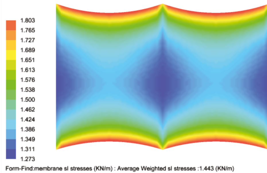
Membrane warp stresses
