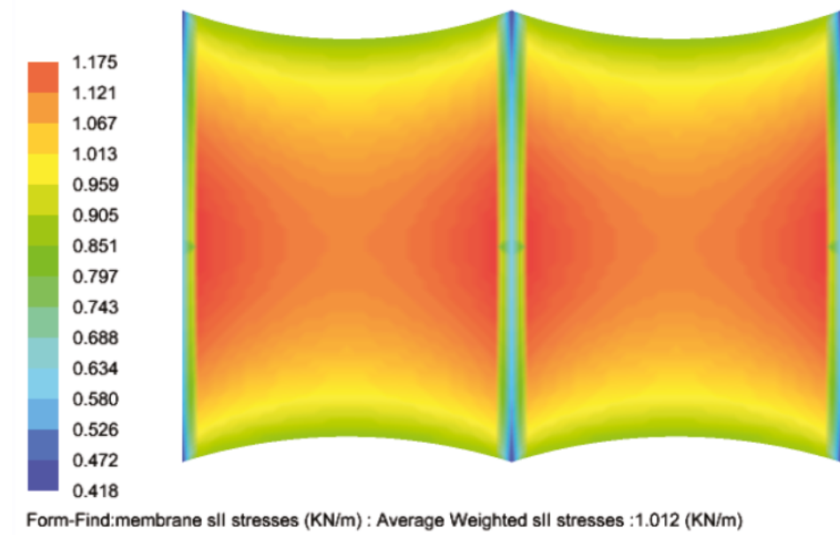
Membrane weft stresses
