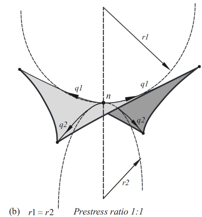
Figure 1.8 Prestress and surface curvature
