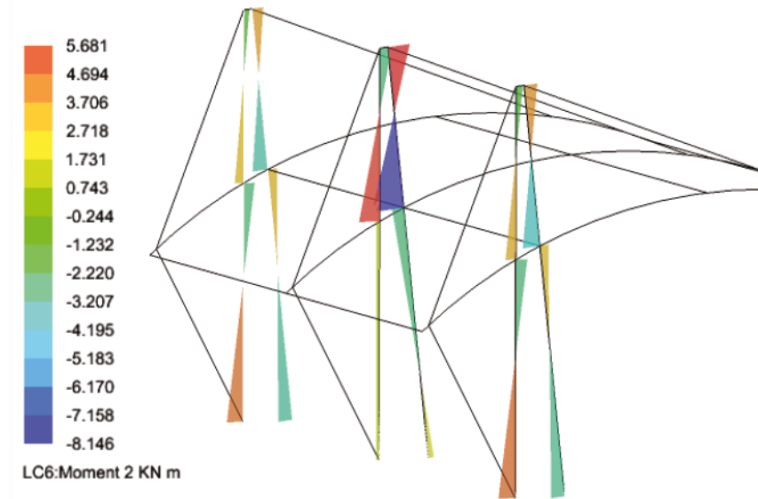
LC6 - Mast M2 reactions
