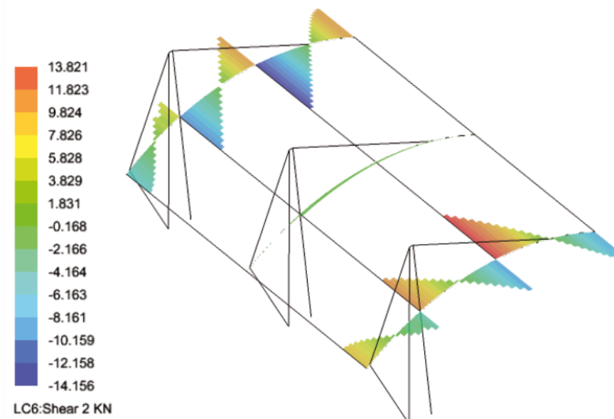
LC6 - Arch shear 2 reactions
