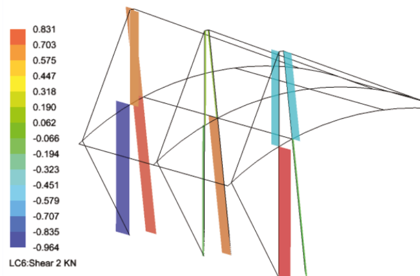
LC6 - Mast shear 2 reactions
