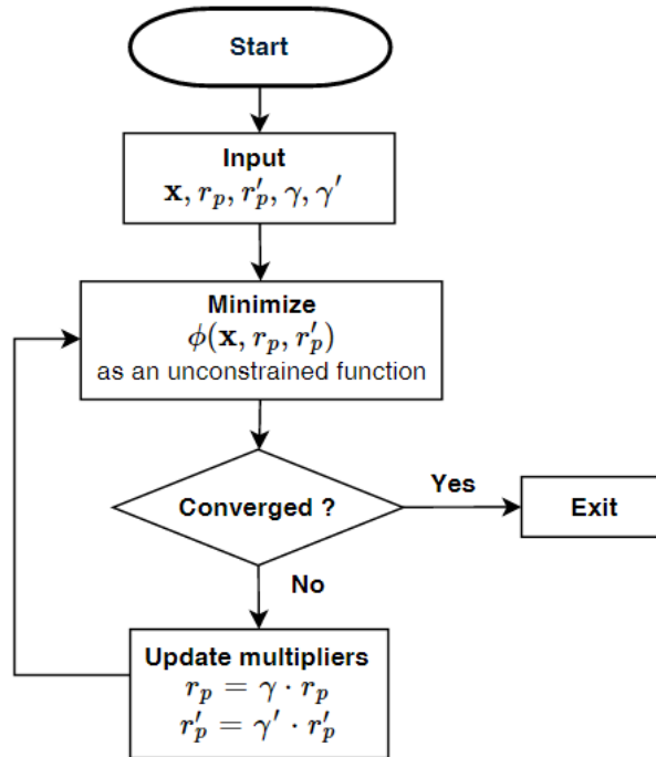
Fig. 34 - Algorithm for barrier (interior penalty function) method
