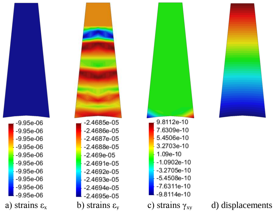
Fig. 19 - Strains resulting from constant compensation
