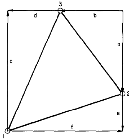
Fig. 2 - Three node constant strain element in local coordinate system
