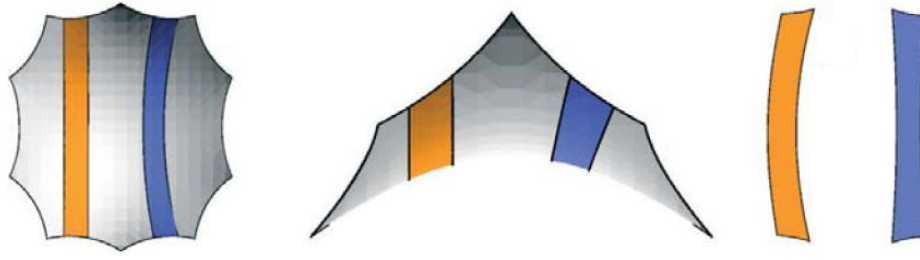
Fig. 9 - Comparison of non-geodesic (orange) and geodesic (blue) cloth generation
