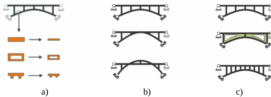
Fig. 21 - Types of structural optimization problems - a) sizing, b) shape, c) topology optimization
