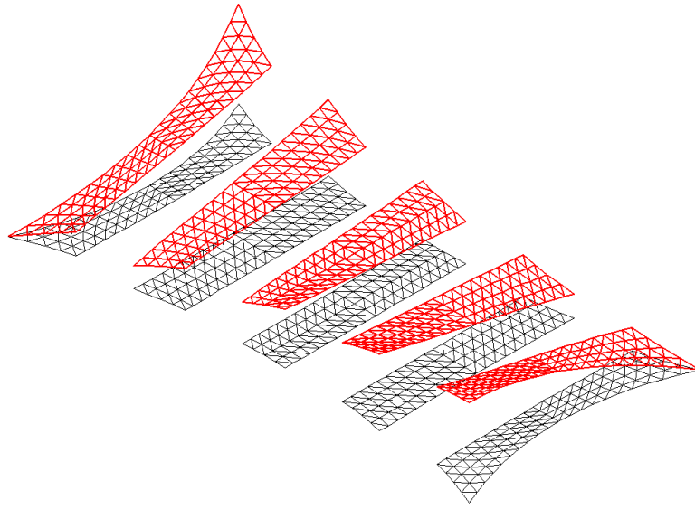
Fig. 17 - Spatial strips and thier planar mapping (initially flattened)
