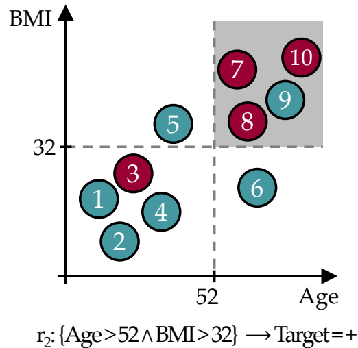
Figure 3.3: Exemplary classification rule. The gray area represents the data space of the covered instances.
