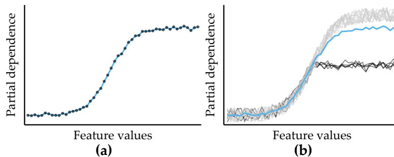
Figure 8.1: Illustrations of a partial dependence plot (PDP) and an individual conditional expectation (ICE) plot on artificial data. (a) PDP for a feature on an artificial dataset. Points represent a sample of the feature distribution. (b) PDP augmented with ICE curves. There are two distinct subsets of observations for which the PD is different in the upper half of the feature distribution.
