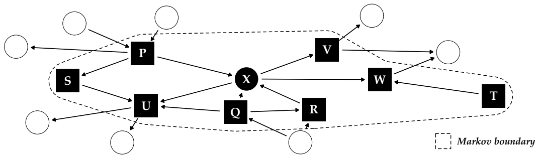
Figure 10.1: Illustrative example of a directed acyclic graph and Markov boundary for the target X . The other labeled variables P - W constitute the Markov boundary of X , consisting of its parents, children and any additional parents of its children (“spouses”).
