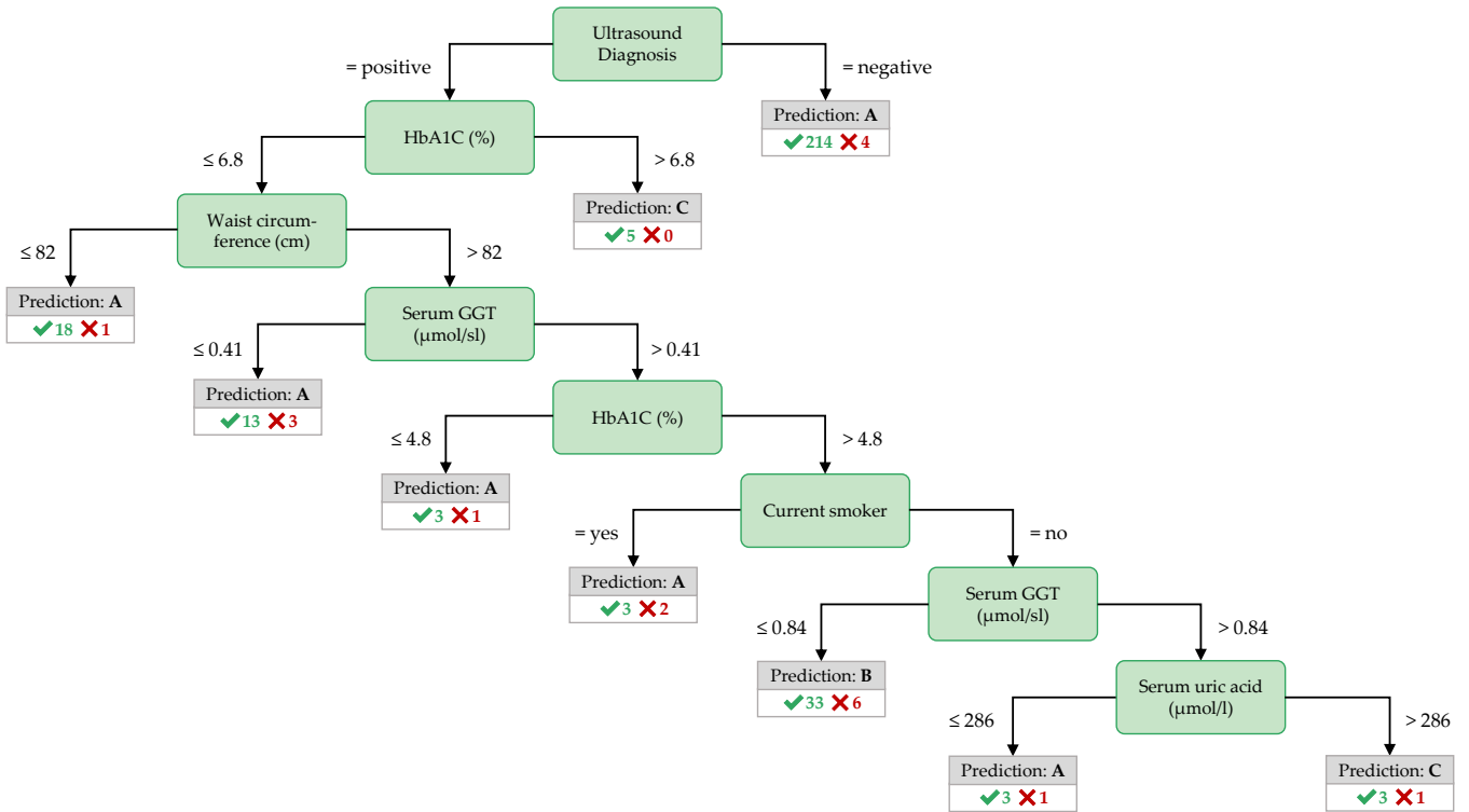
Figure 3.8: Best decision tree for PartitionF, achieved by the variant InfoGain .
