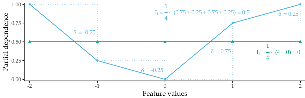
Figure 8.3: Illustration of partial dependence importance. Partial dependence importance I_f for two exemplary PD curves.
