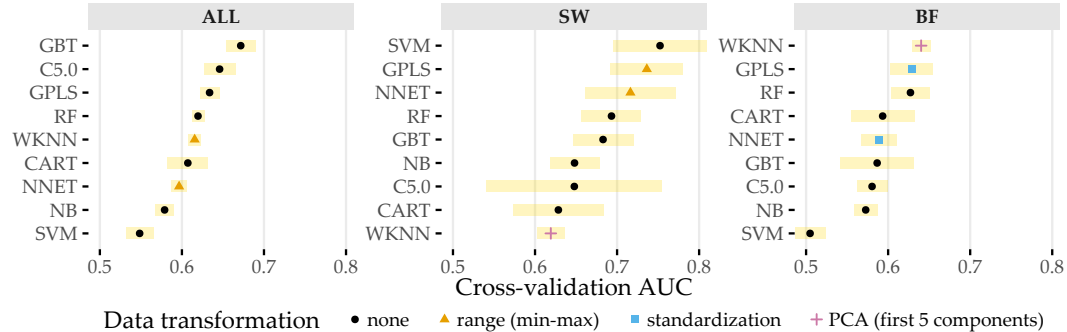
Figure 8.12: Classification results for ANEUR. For each combination of data subset and classification algorithm, the performance of the run with the preprocessing transformation that achieves the highest AUC is shown. SW = sidewall; BF = bifurcation.
