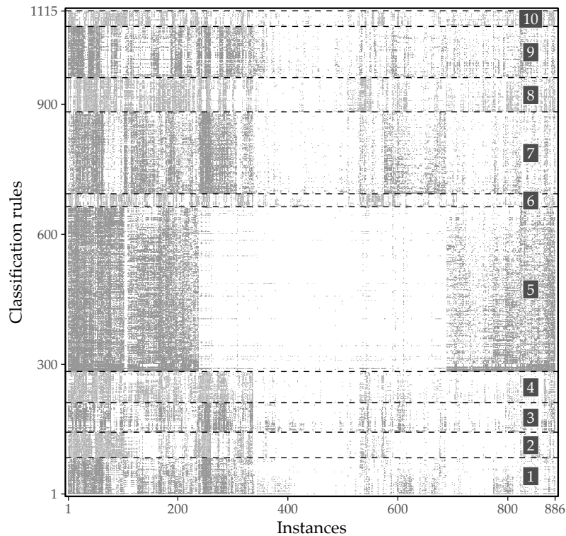
Figure 4.2: Illustration of rule redundancy. Graphical representation of 1115 HotSpot rules found on SHIP data on 886 labeled instances. A gray cell indicates that the instance at that x-position is covered by the rule at the associated y-position. Instances and rules are sorted by agglomerative hierarchical clustering. When partitioning into 10 clusters based on the covered instances, each cluster’s rules describe similar subpopulations.
