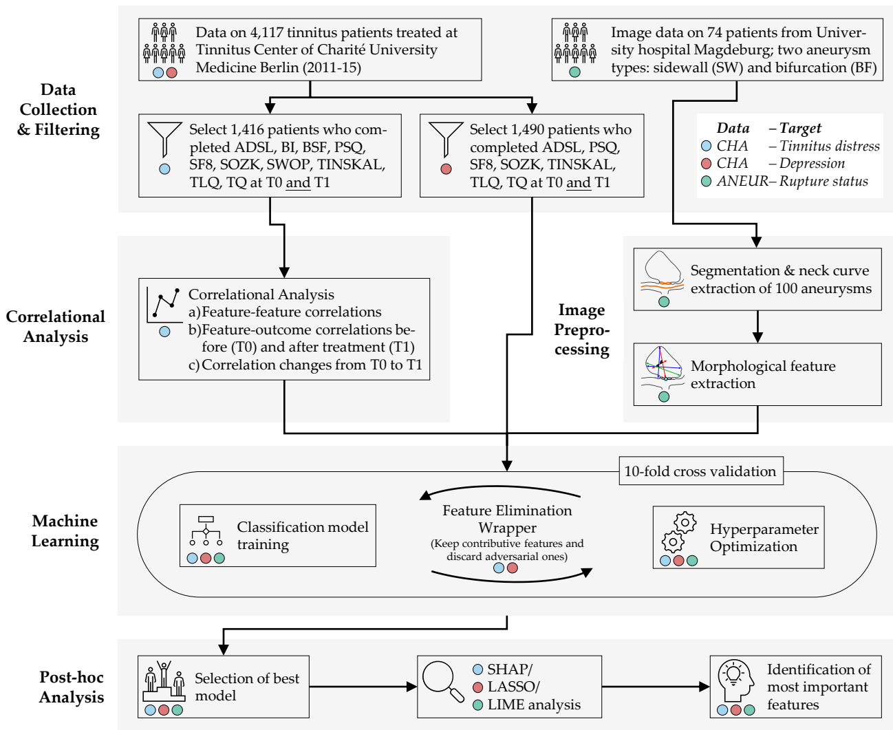
Figure 8.4: The (dataset-specific) mining workflow. For the CHA dataset, we select patients with complete data for each of the two classification tasks. For ANEUR, we segment the aneurysms from the raw image data, perform automated centerline and neck curve extraction, and generate the morphological features. We perform correlation analysis to identify relevant correlations between features, correlations between features and target variable, and significant differences in correlation between features and target variable between T0 and T1. We embed model training in an iterative feature elimination wrapper that retains features identified as important to the model. We select the best overall model based on AUC and used post-hoc interpretation methods to identify features with the highest attribution to the model prediction on a global, subpopulation and observation level.
