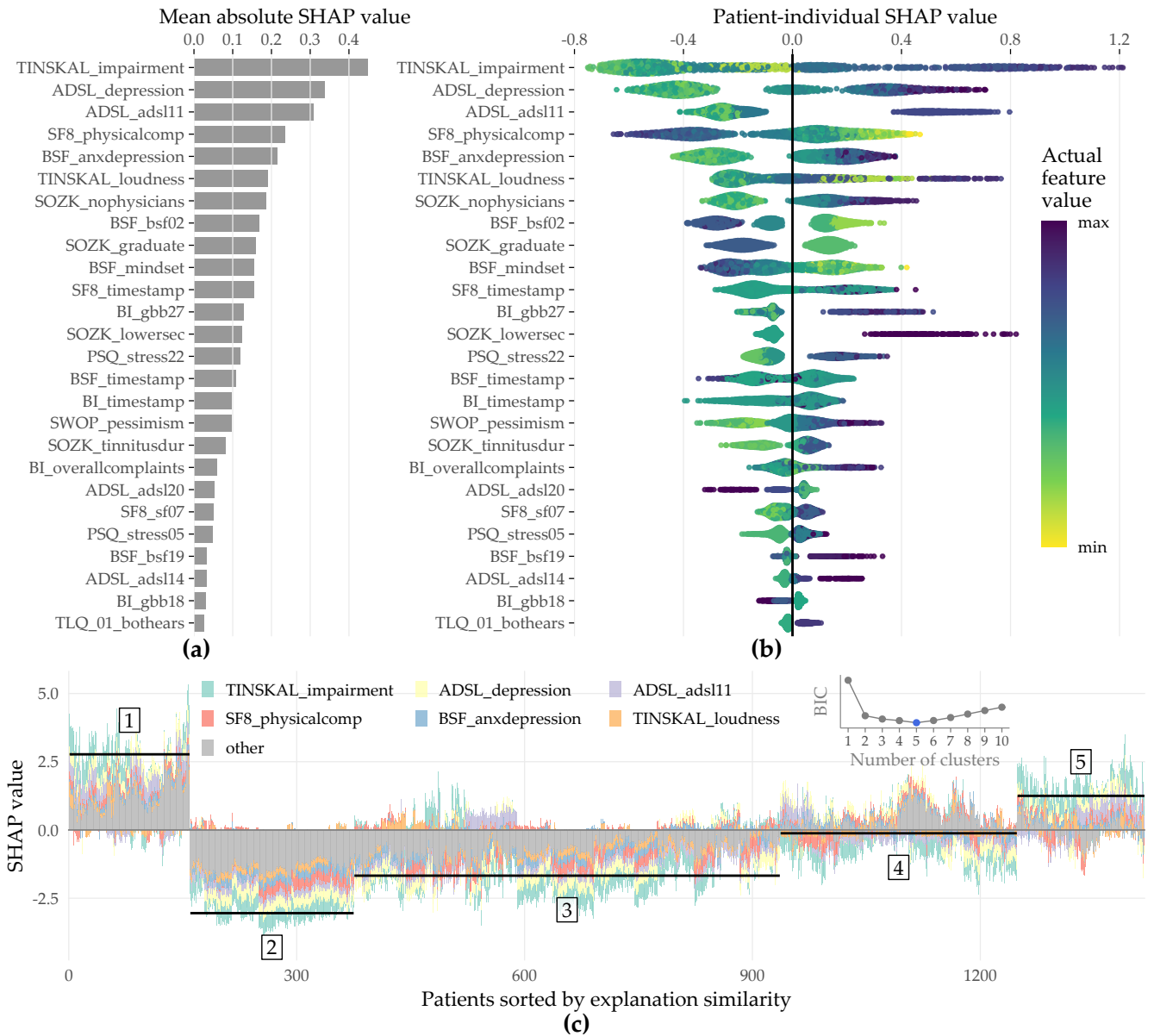
Figure 8.7: SHAP analysis results for the best model (GBT, feature elimination iteration i = 7 ). (a) Global feature importance based on the mean absolute SHAP magnitude over all observations. Values depict the absolute change in log odds where higher values indicate higher feature attribution towards the model. (b) Patient-individual SHAP values. A point represents the SHAP value of the feature (y-axis) for an individual patient. The further a point from the vertical 0-baseline, the larger the attribution of the corresponding feature value to the model prediction. Vertically offset points depict high-density regions (similar to a violin plot), i.e., there are more patients with similar SHAP values. Actual feature values are mapped to point color. (c) Stacked patient-individual SHAP values for the six features with the highest mean absolute SHAP values. Patients are ordered according to hierarchical clustering with Ward linkage. Black horizontal lines depict the average sum of SHAP values of the cluster members for k = 5 clusters. The inset plot shows that the Bayesian information criterion (BIC) is minimal for this number of clusters.
