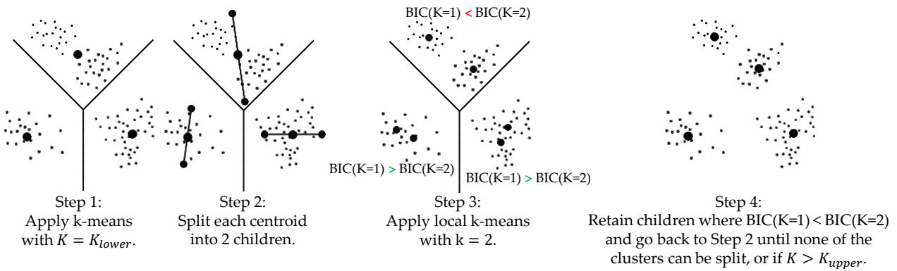
Figure 5.1: Principal steps of X-means (simplified) . The figure is adapted from [PMoo].
