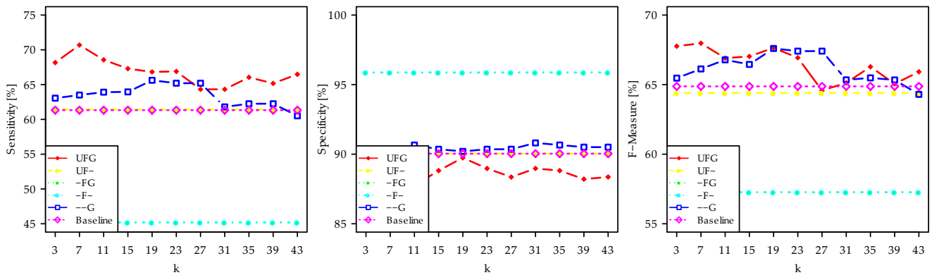
Figure 6.4: Comparison of classification performance for workflow components. Sensitivity (left), specificity (center) and F-measure scores (right) for each workflow variant and the baseline using decision tree for learning. The figure is adapted from [Nie+15].
