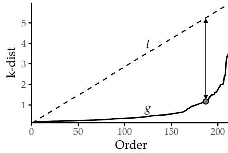
Figure 6.2: Setting \text{eps} based on the k-dist graph for a given \text{minPts} . The k-dist graph g depicts the sorted distances to the points' k th next neighbors. A suitable \text{eps}_{\text{opt}} can be identified with the maximum distance between the k-dist and the line l that connects the first and the last point of g . For DBSCAN clustering with \text{minPts} = k , \text{eps}_{\text{opt}} , points with \text{k-dist} \leq \text{eps}_{\text{opt}} will become core points, else border or noise points.
