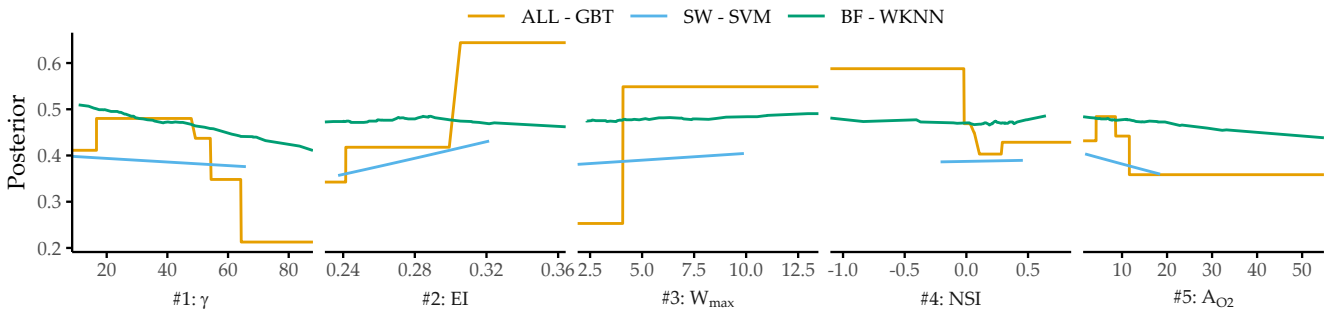
Figure 8.16: PDP curves for top 5 features on ALL - GBT for each data subset's best model.
