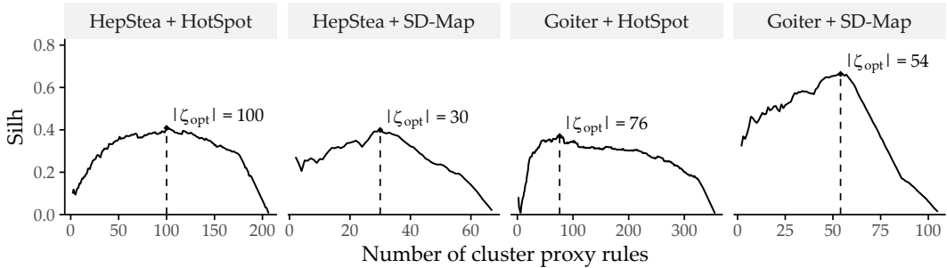
Figure 4.3: Silhouette coefficients (Silh) of SD-Clu using complete linkage for each combination of dataset and algorithm. The number of clusters k with the highest Silh score ( |\zeta_{\text{opt}}| ) is indicated by a dashed vertical line.
