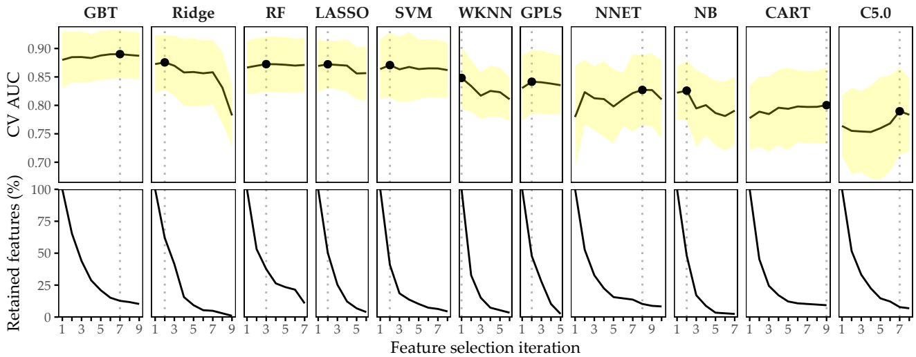
Figure 8.6: Classification results for CHA-Tinnitus. Average cross-validation AUC and relative number of retained features for each classifier with optimal hyperparameter configuration and each feature selection iteration. Yellow ribbons depict standard deviation. Points highlight each classifier’s run with maximum AUC. Classifiers are ordered by their maximum AUC from left to right.
