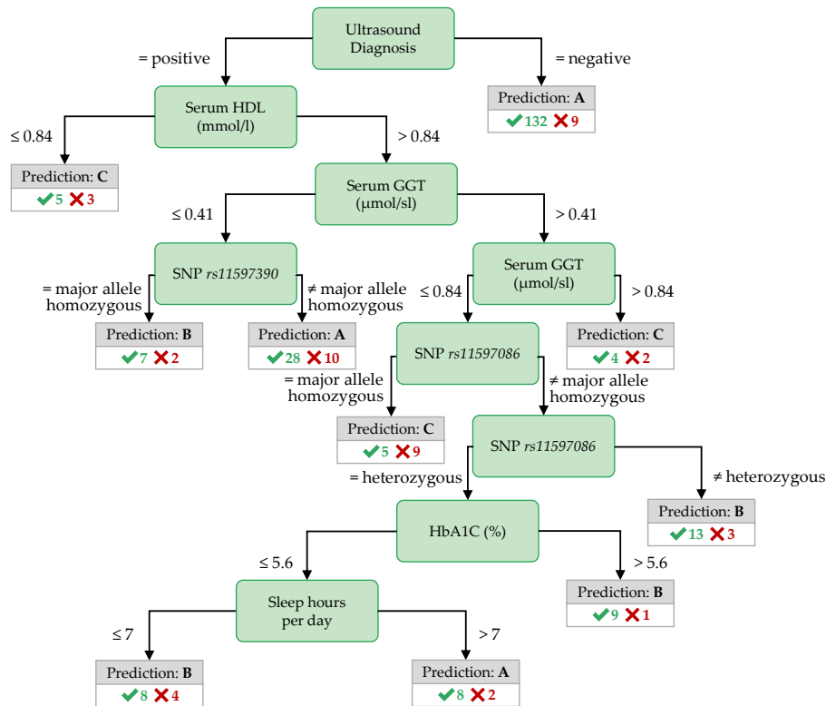
Figure 3.9: Best decision tree for PartitionM , achieved by the variant CostMatrix .
