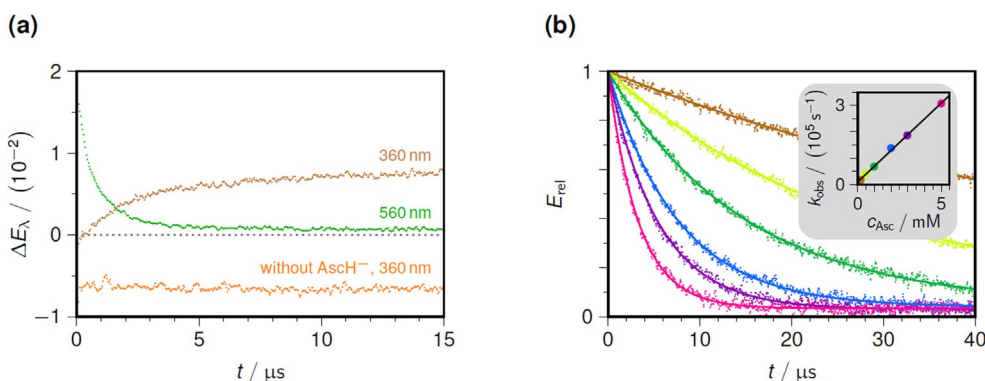
Figure 4. Repair of the quercetin radical (about 2.1 \mu\text{M} ) by ascorbate in homogeneous aqueous solution saturated with \text{N}_2\text{O} . Graph (a): extinction traces \Delta E used for calibrating \epsilon_{\text{max}} of \text{Q}^{\cdot-} ; pH 6.5; ascorbate weight-in concentration, 100 mM and 0 mM (control experiment). Green trace, 560 nm; detection of \text{Q}^{\cdot-} . Brown and orange traces, 360 nm; superposition of (starting) quercetin depletion, \text{Q}^{\cdot-} decay, and \text{Asc}^{\cdot-} formation (not in the control experiment without ascorbate). The dotted gray line ( \Delta E = 0 ) serves to guide the eye. Graph (b): dependence of the observed repair rate constant k_{\text{obs}} on the ascorbate weight-in concentration c_{\text{Asc}} (color-coded identically in the main plot and the inset) at pH 4.25. Main plot, decay curves of the quercetin radicals, measured through the extinctions E_{\text{rel}} (at 515 nm, each curve normalized to the initial post-flash value) with overlaid best fits of pseudo first-order decays to a residual floor; inset, Stern–Volmer plot giving an apparent bimolecular rate constant of 6.0 \times 10^7 \text{ M}^{-1} \text{ s}^{-1} . For further explanation, see the text.
