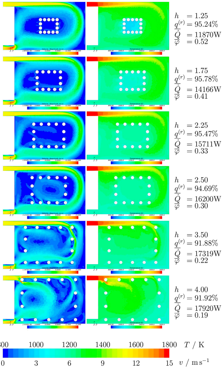
FIGURE 7 | Velocity magnitude (left column) and temperature fields (right column) for the configuration D at different distance factors with an inner tube radius of r = 0.063 m, and a flue gas mass flow of \dot{m}_{fl} = 0.03 kg/s/tube.
