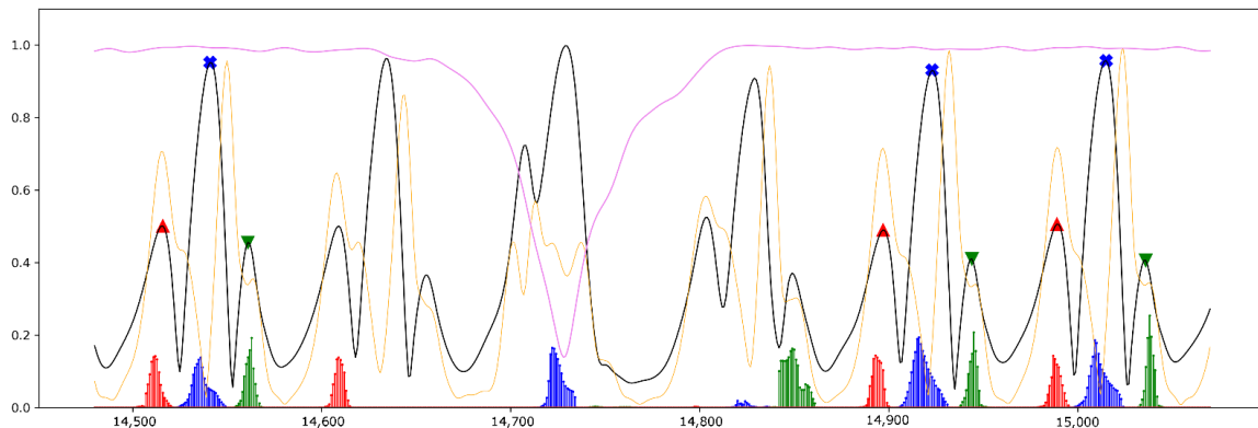
Figure 7. A short part of the evaluation results from Test_1_G. This figure shows six steps while walking straight forward, turning at the end of the walking track, and then walking back. Black line: smoothed AngVelMag; orange line: smoothed FreeAccMag; violet line: smoothed RotMatMag, red markers: labeled FO; red vertical lines: predictions for FO; blue markers: labeled MidS; blue vertical lines: predictions for MidS; green marker: labeled FC; green vertical lines: predictions for FC.
