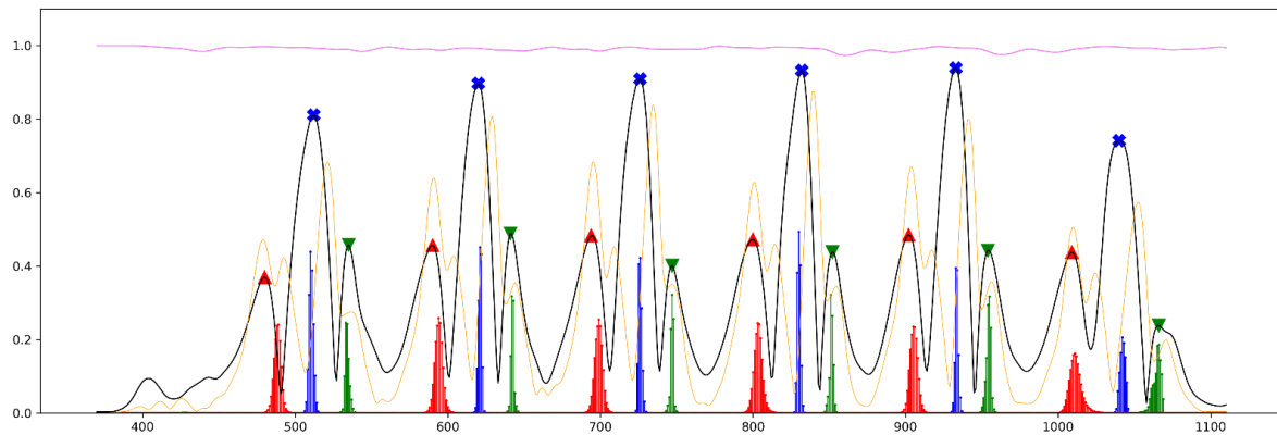
Figure 6. A short part of the prediction results from Test_2_H. This figure demonstrates six steps from the beginning of walking till the last step before turning at the end of the walking track. Black line: smoothed AngVelMag; orange line: smoothed FreeAccMag; violet line: smoothed RotMatMag, red markers: labeled FO; red vertical lines: predictions for FO; blue markers: labeled MidS; blue vertical lines: predictions for MidS; green marker: labeled FC; green vertical lines: predictions for FC.
